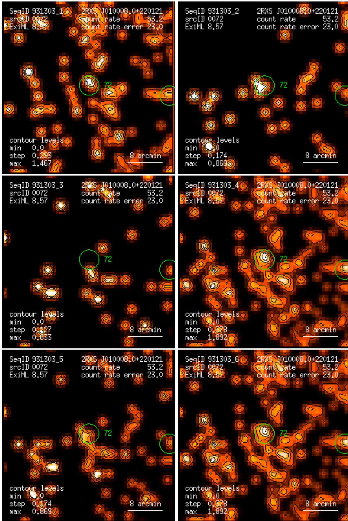
Figure 72: RASS 931303: detection 0072: band rate images, Gaussian filter: (1) PSPC channels 11 – 41, (2) 52 – 90, (3) 91 – 201, (4) 11 – 235, (5) 52 – 201, (6) 11 – 201. Broad band rates in counts/ks. Band rate contour levels in counts/ks/arcmin 2 .
