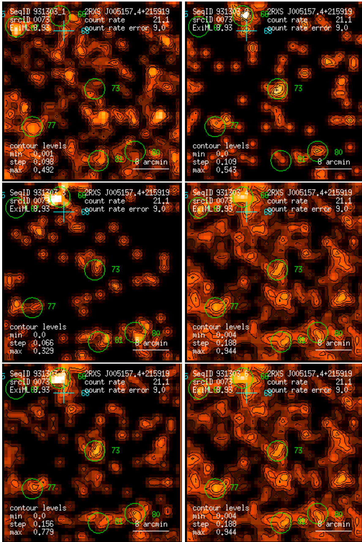
Figure 73: RASS 931303: detection 0073: band rate images, Gaussian filter: (1) PSPC channels 11 – 41, (2) 52 – 90, (3) 91 – 201, (4) 11 – 235, (5) 52 – 201, (6) 11 – 201. Broad band rates in counts/ks. Band rate contour levels in counts/ks/arcmin 2 .
