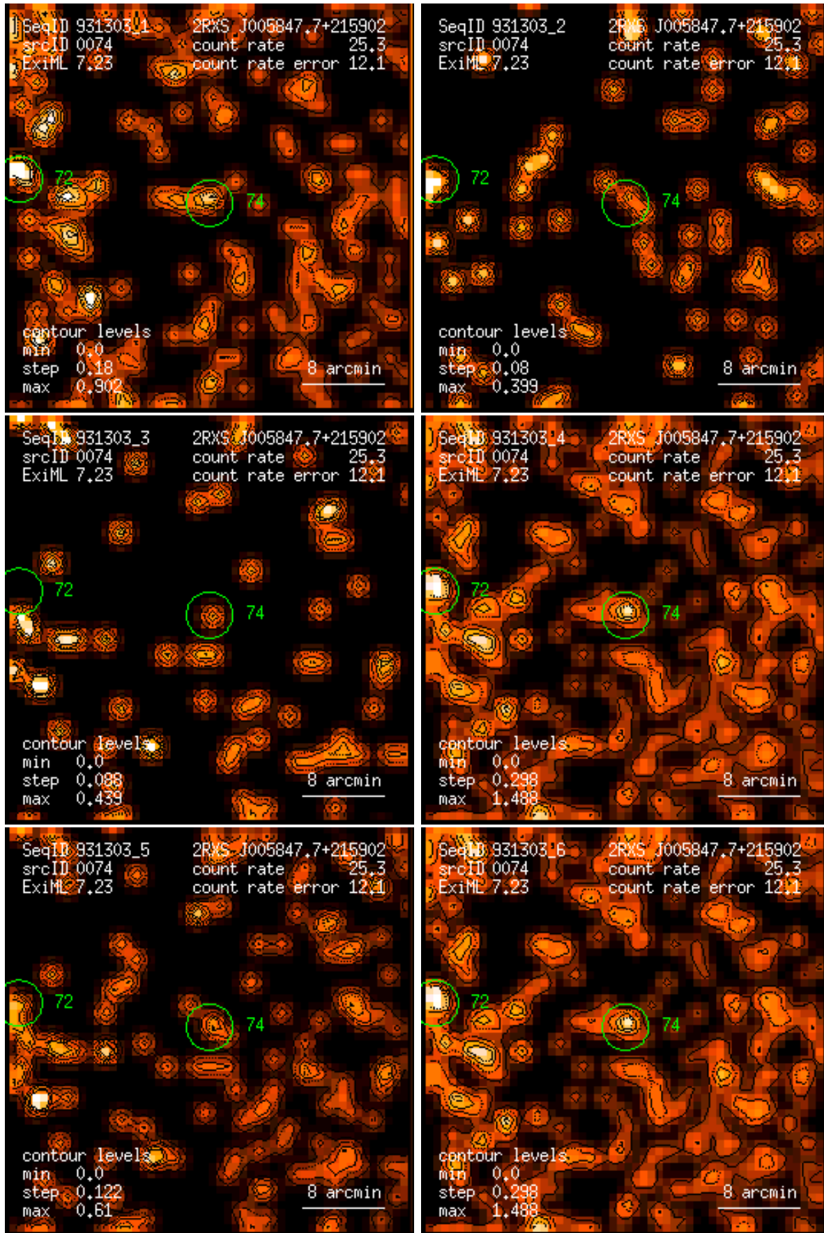
Figure 74: RASS 931303: detection 0074: band rate images, Gaussian filter: (1) PSPC channels 11 – 41, (2) 52 – 90, (3) 91 – 201, (4) 11 – 235, (5) 52 – 201, (6) 11 – 201. Broad band rates in counts/ks. Band rate contour levels in counts/ks/arcmin 2 .
