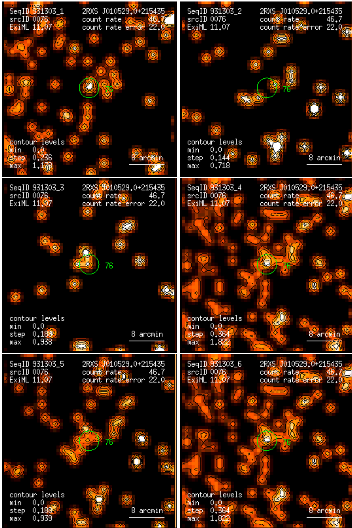
Figure 76: RASS 931303: detection 0076: band rate images, Gaussian filter: (1) PSPC channels 11 – 41, (2) 52 – 90, (3) 91 – 201, (4) 11 – 235, (5) 52 – 201, (6) 11 – 201. Broad band rates in counts/ks. Band rate contour levels in counts/ks/arcmin 2 .
