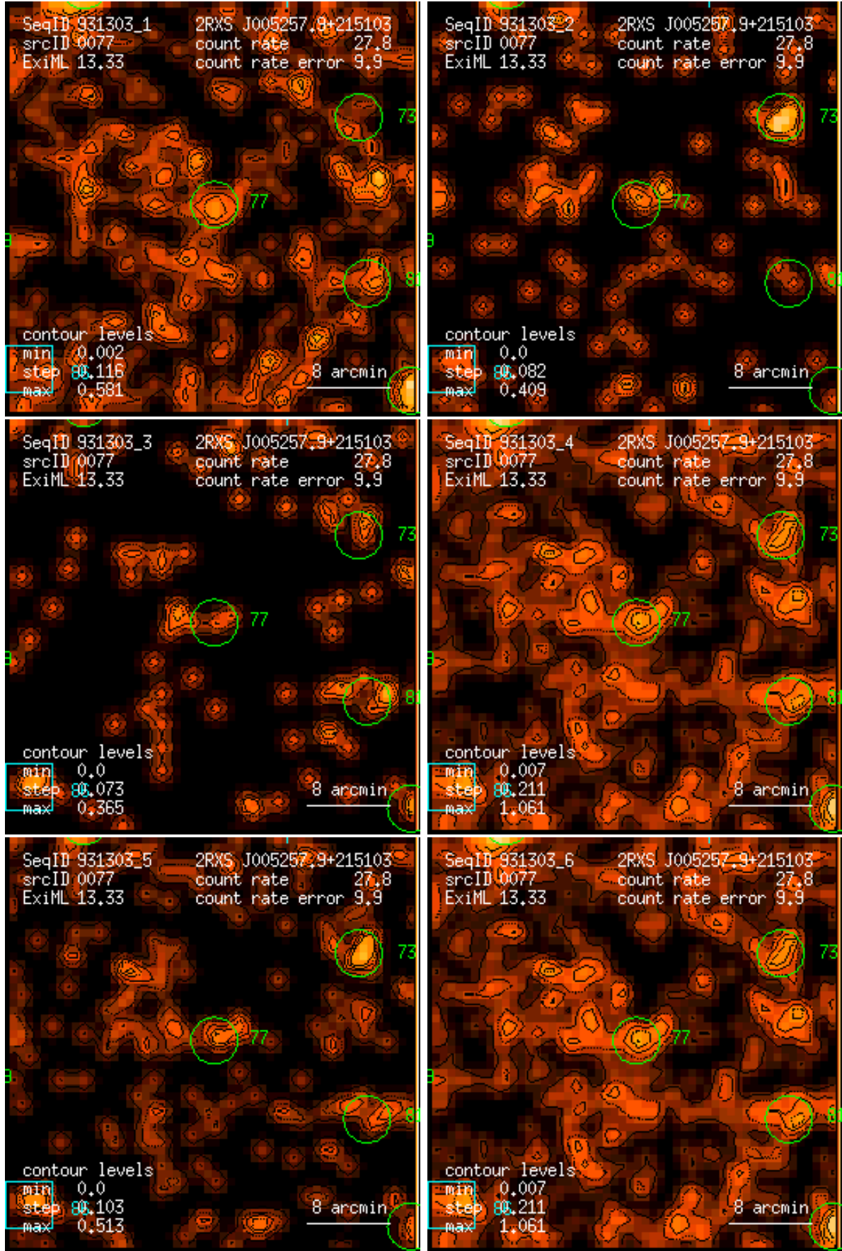
Figure 77: RASS 931303: detection 0077: band rate images, Gaussian filter: (1) PSPC channels 11 – 41, (2) 52 – 90, (3) 91 – 201, (4) 11 – 235, (5) 52 – 201, (6) 11 – 201. Broad band rates in counts/ks. Band rate contour levels in counts/ks/arcmin 2 .
