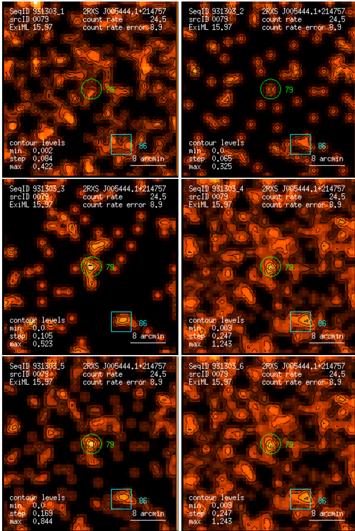
Figure 79: RASS 931303: detection 0079: band rate images, Gaussian filter: (1) PSPC channels 11 – 41, (2) 52 – 90, (3) 91 – 201, (4) 11 – 235, (5) 52 – 201, (6) 11 – 201. Broad band rates in counts/ks. Band rate contour levels in counts/ks/arcmin 2 .
