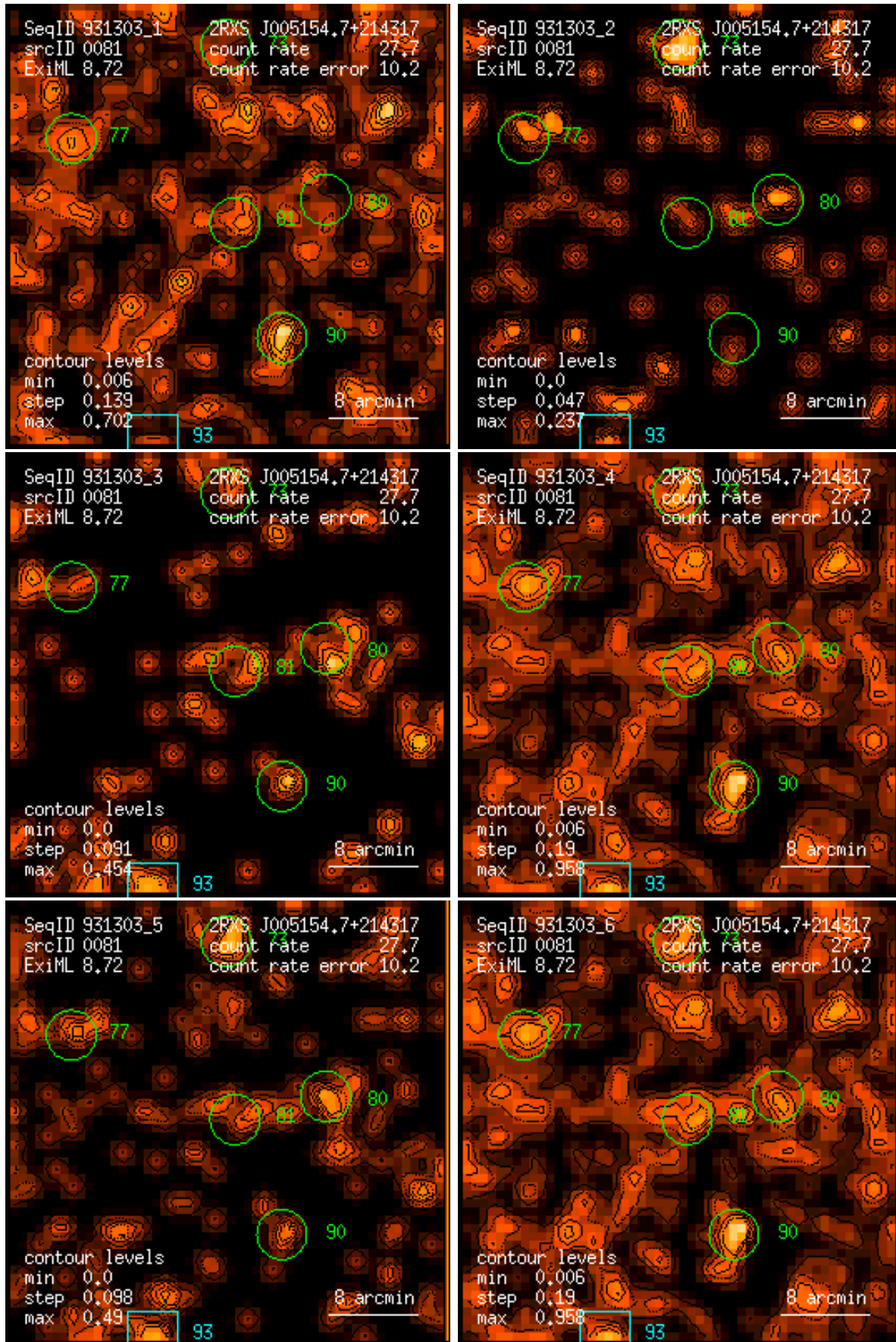
Figure 81: RASS 931303: detection 0081: band rate images, Gaussian filter: (1) PSPC channels 11 – 41, (2) 52 – 90, (3) 91 – 201, (4) 11 – 235, (5) 52 – 201, (6) 11 – 201. Broad band rates in counts/ks. Band rate contour levels in counts/ks/arcmin 2 .
