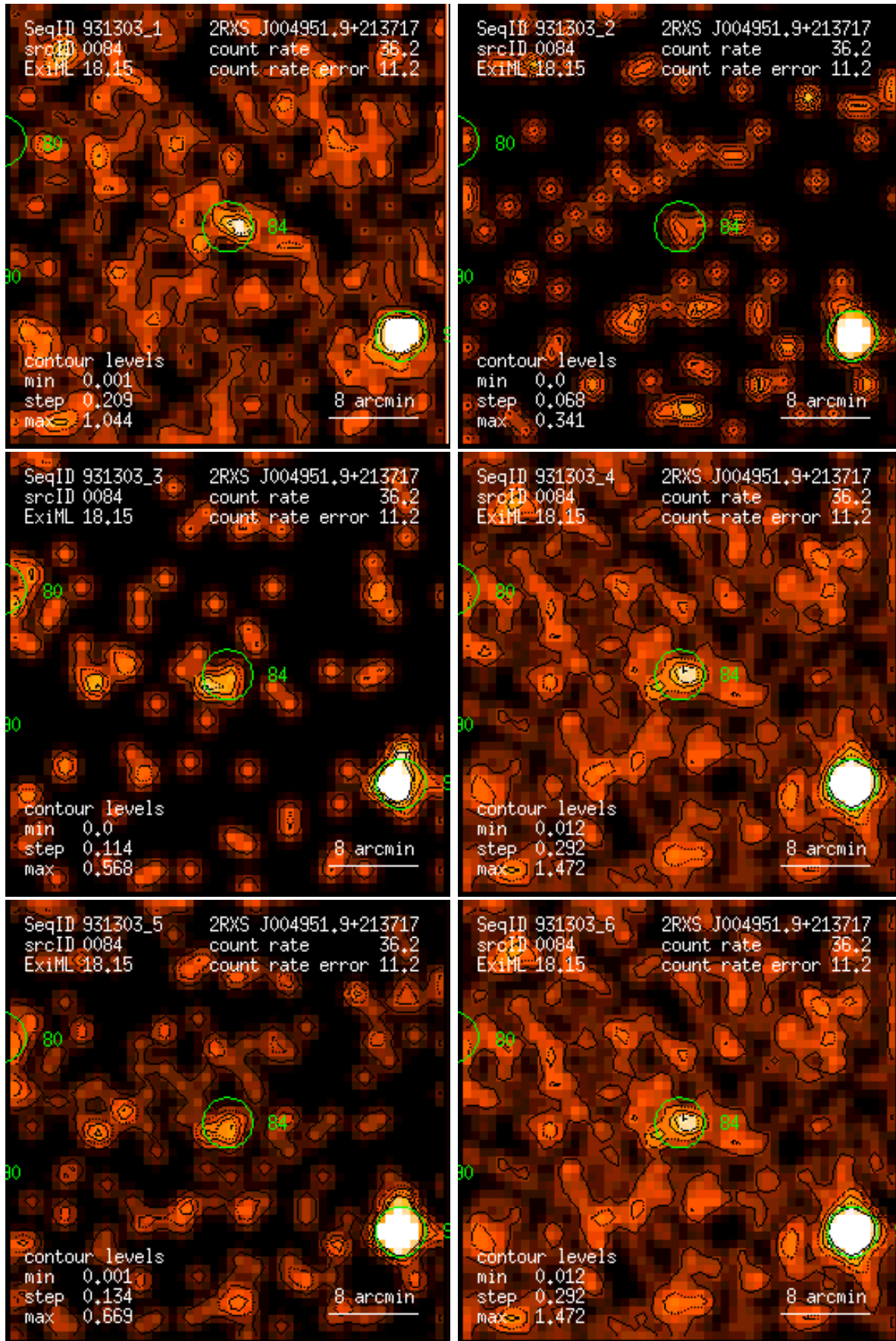
Figure 84: RASS 931303: detection 0084: band rate images, Gaussian filter: (1) PSPC channels 11 – 41, (2) 52 – 90, (3) 91 – 201, (4) 11 – 235, (5) 52 – 201, (6) 11 – 201. Broad band rates in counts/ks. Band rate contour levels in counts/ks/arcmin 2 .
