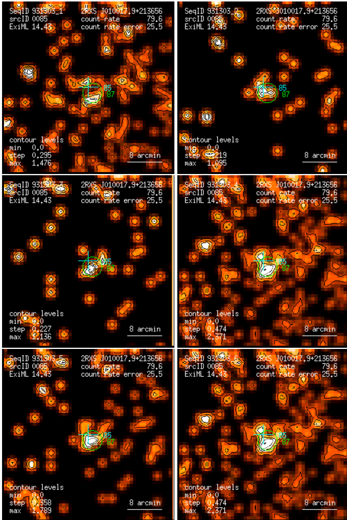
Figure 85: RASS 931303: detection 0085: band rate images, Gaussian filter: (1) PSPC channels 11 – 41, (2) 52 – 90, (3) 91 – 201, (4) 11 – 235, (5) 52 – 201, (6) 11 – 201. Broad band rates in counts/ks. Band rate contour levels in counts/ks/arcmin 2 .
