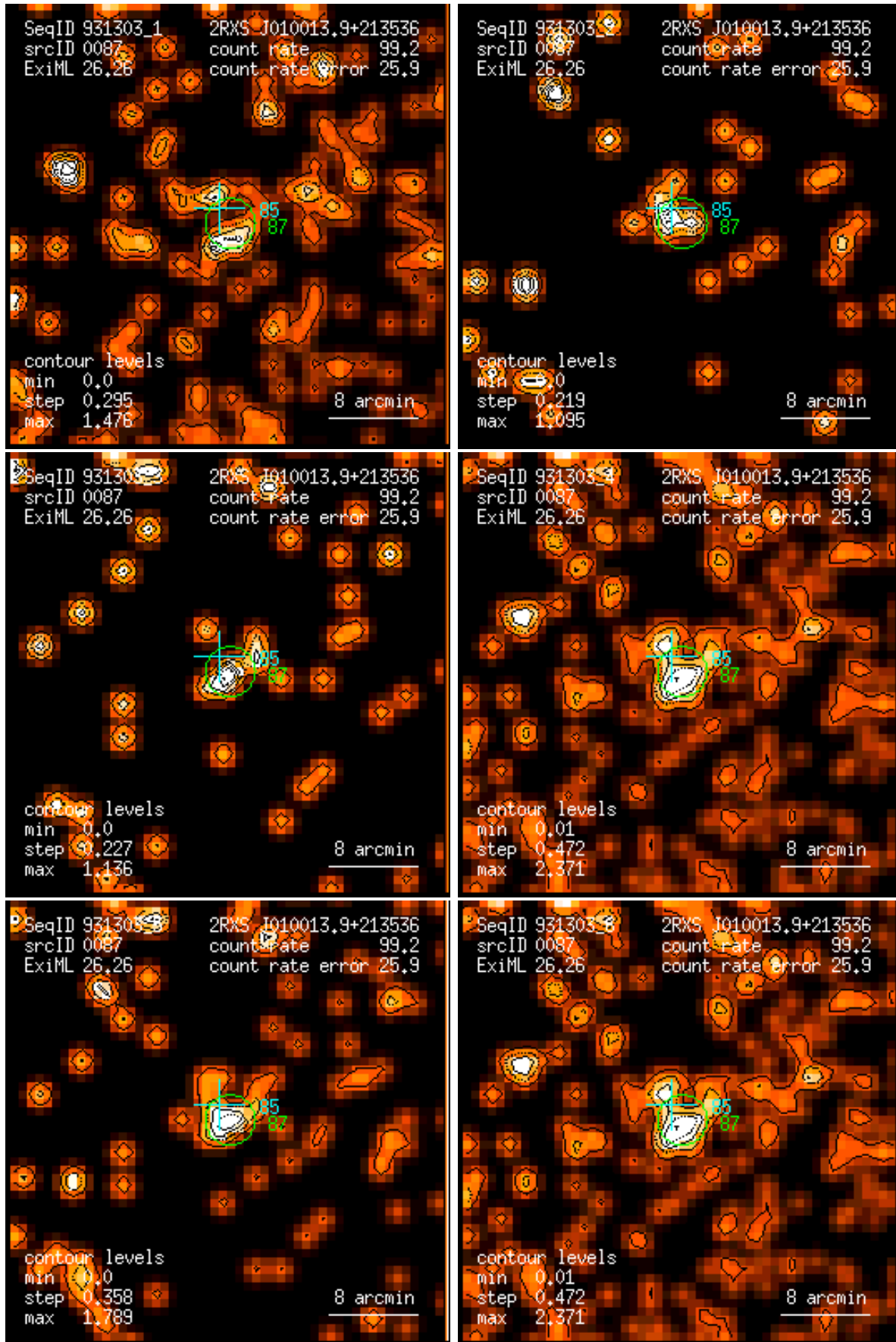
Figure 87: RASS 931303: detection 0087: band rate images, Gaussian filter: (1) PSPC channels 11 – 41, (2) 52 – 90, (3) 91 – 201, (4) 11 – 235, (5) 52 – 201, (6) 11 – 201. Broad band rates in counts/ks. Band rate contour levels in counts/ks/arcmin 2 .
