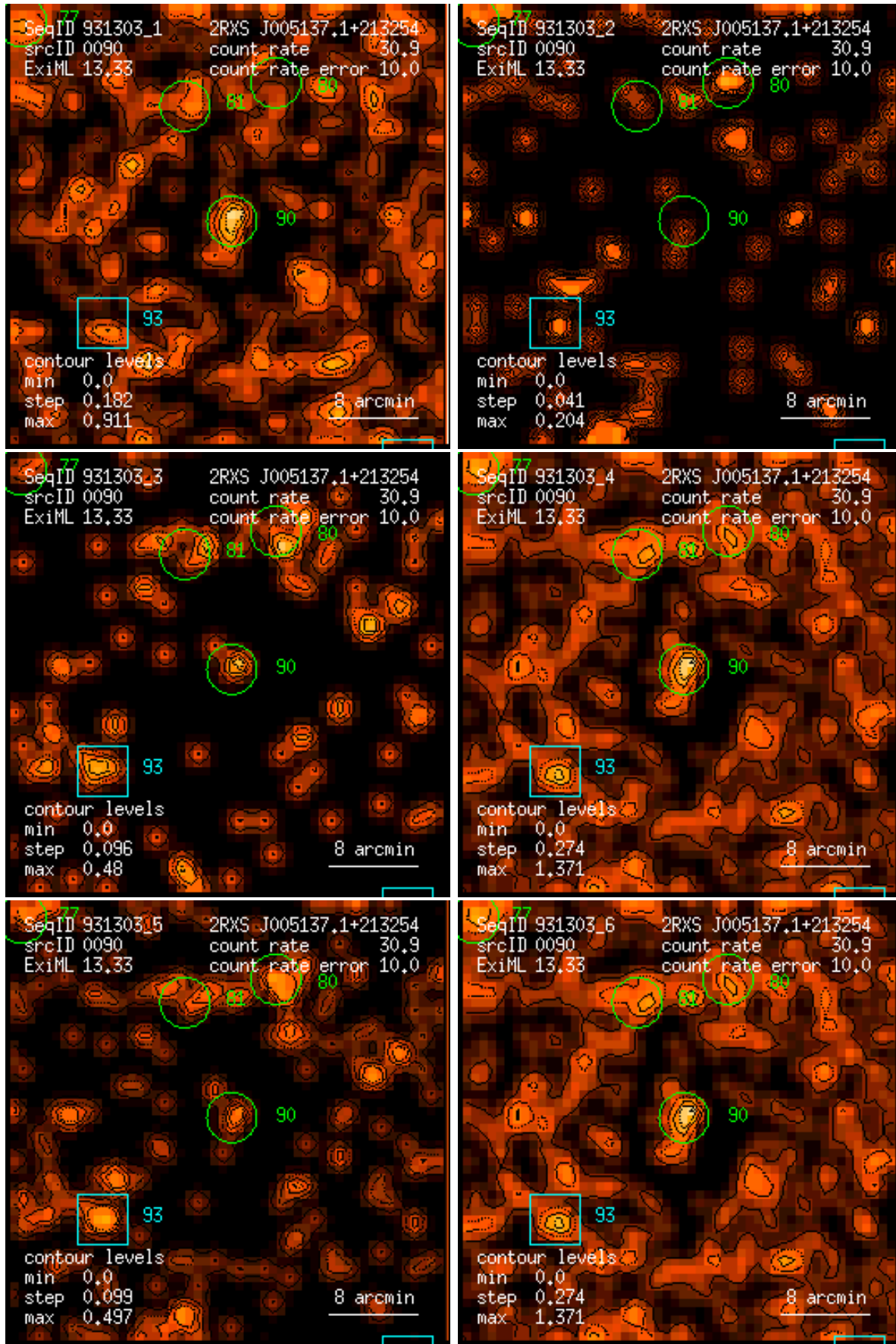
Figure 90: RASS 931303: detection 0090: band rate images, Gaussian filter: (1) PSPC channels 11 – 41, (2) 52 – 90, (3) 91 – 201, (4) 11 – 235, (5) 52 – 201, (6) 11 – 201. Broad band rates in counts/ks. Band rate contour levels in counts/ks/arcmin 2 .
