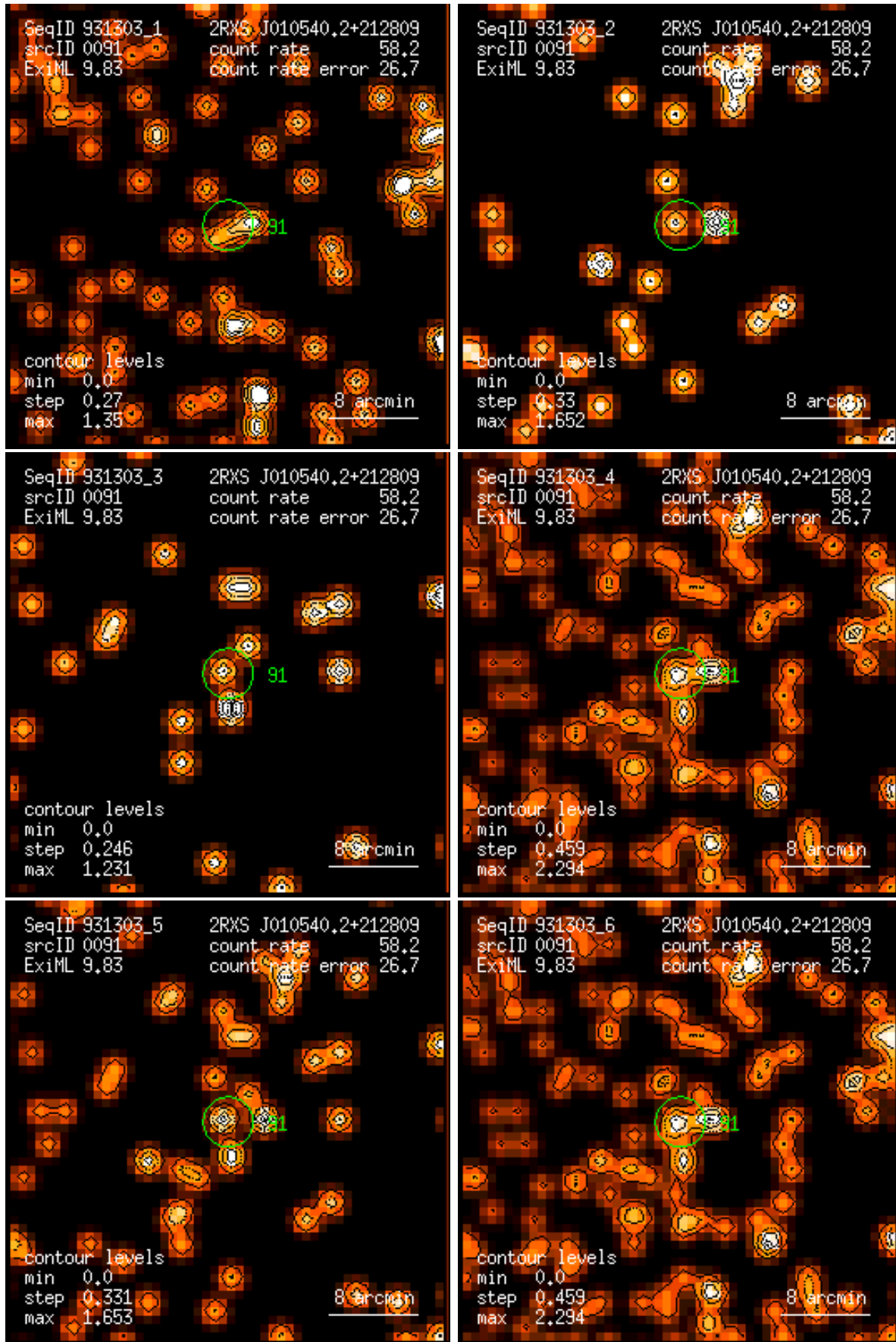
Figure 91: RASS 931303: detection 0091: band rate images, Gaussian filter: (1) PSPC channels 11 – 41, (2) 52 – 90, (3) 91 – 201, (4) 11 – 235, (5) 52 – 201, (6) 11 – 201. Broad band rates in counts/ks. Band rate contour levels in counts/ks/arcmin 2 .
