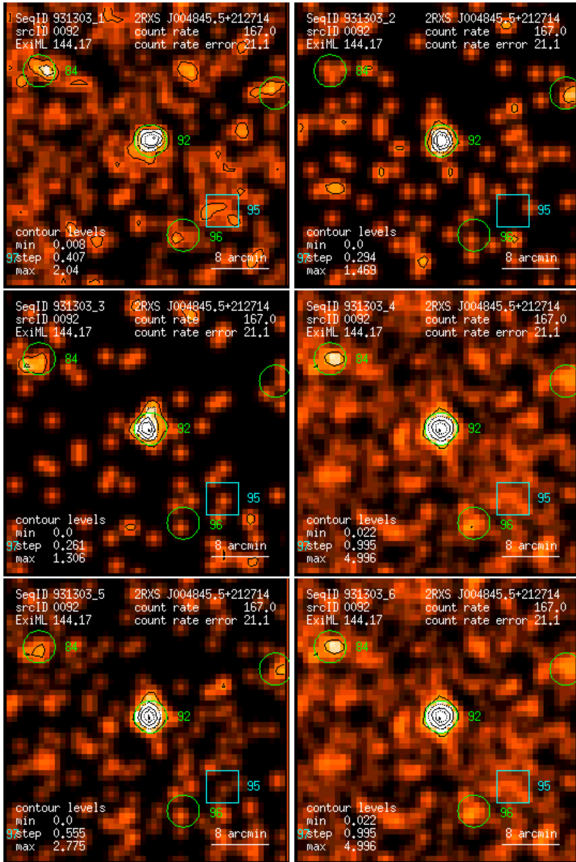
Figure 92: RASS 931303: detection 0092: band rate images, Gaussian filter: (1) PSPC channels 11 – 41, (2) 52 – 90, (3) 91 – 201, (4) 11 – 235, (5) 52 – 201, (6) 11 – 201. Broad band rates in counts/ks. Band rate contour levels in counts/ks/arcmin 2 .
