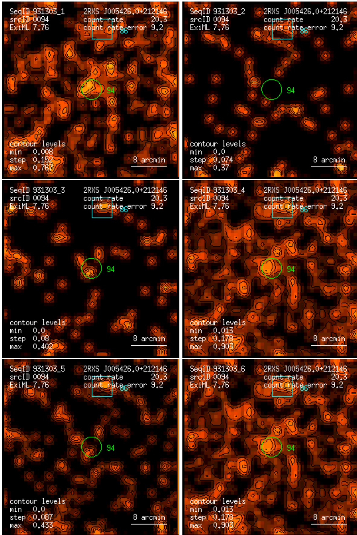
Figure 94: RASS 931303: detection 0094: band rate images, Gaussian filter: (1) PSPC channels 11 – 41, (2) 52 – 90, (3) 91 – 201, (4) 11 – 235, (5) 52 – 201, (6) 11 – 201. Broad band rates in counts/ks. Band rate contour levels in counts/ks/arcmin 2 .
