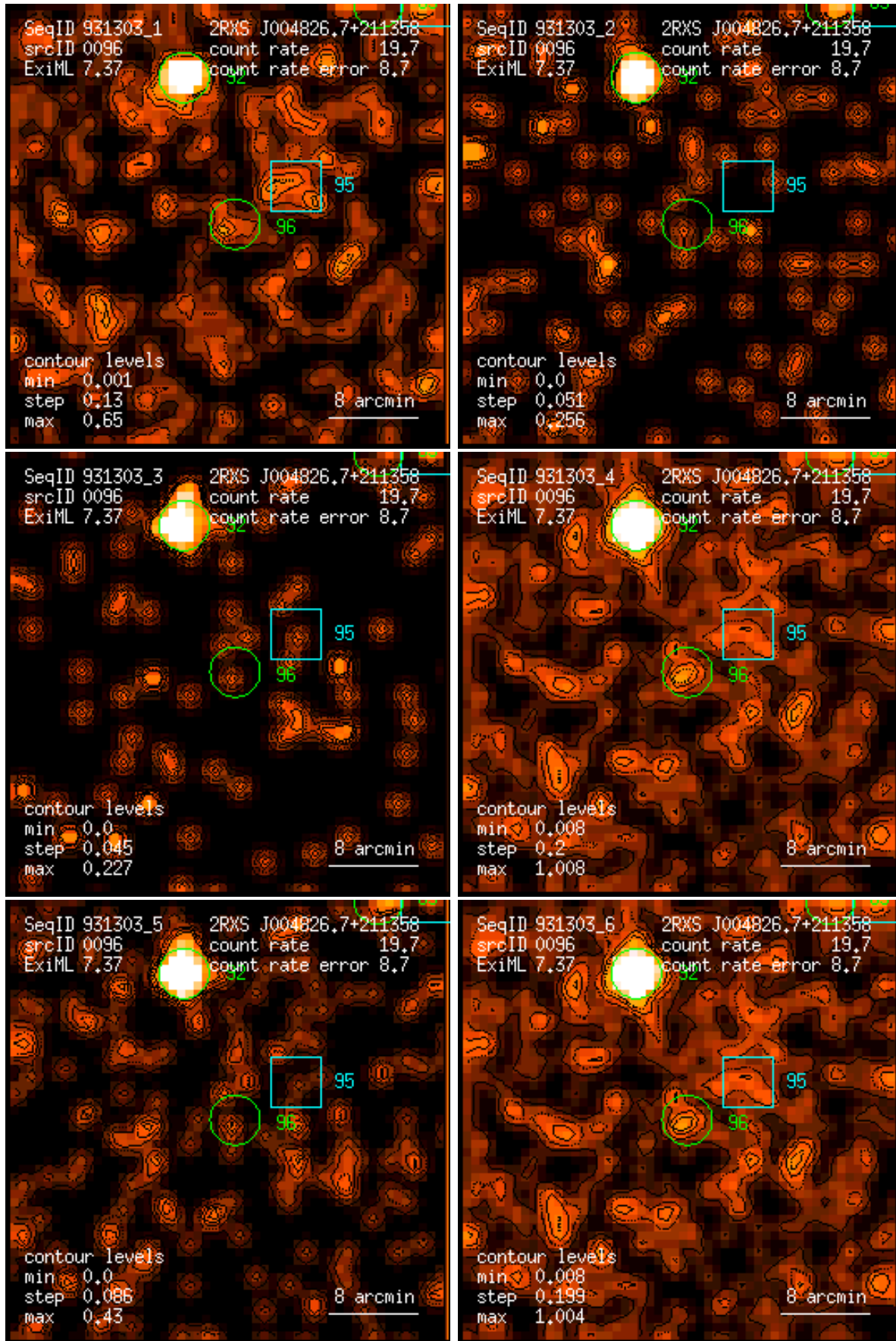
Figure 96: RASS 931303: detection 0096: band rate images, Gaussian filter: (1) PSPC channels 11 – 41, (2) 52 – 90, (3) 91 – 201, (4) 11 – 235, (5) 52 – 201, (6) 11 – 201. Broad band rates in counts/ks. Band rate contour levels in counts/ks/arcmin 2 .
