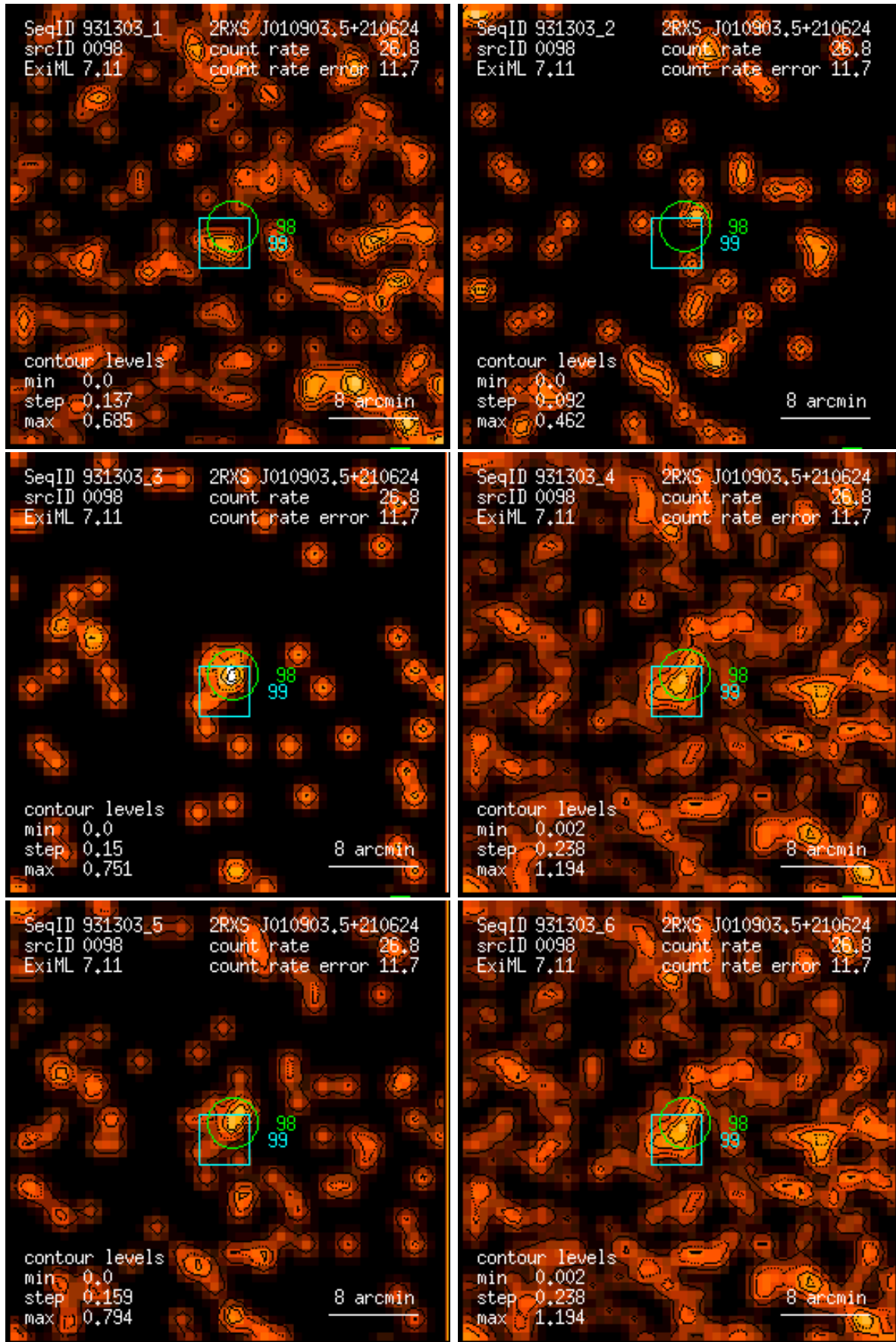
Figure 98: RASS 931303: detection 0098: band rate images, Gaussian filter: (1) PSPC channels 11 – 41, (2) 52 – 90, (3) 91 – 201, (4) 11 – 235, (5) 52 – 201, (6) 11 – 201. Broad band rates in counts/ks. Band rate contour levels in counts/ks/arcmin 2 .
