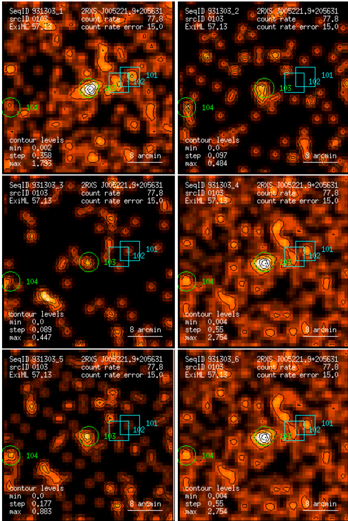
Figure 103: RASS 931303: detection 0103: band rate images, Gaussian filter: (1) PSPC channels 11 – 41, (2) 52 – 90, (3) 91 – 201, (4) 11 – 235, (5) 52 – 201, (6) 11 – 201. Broad band rates in counts/ks. Band rate contour levels in counts/ks/arcmin 2 .
