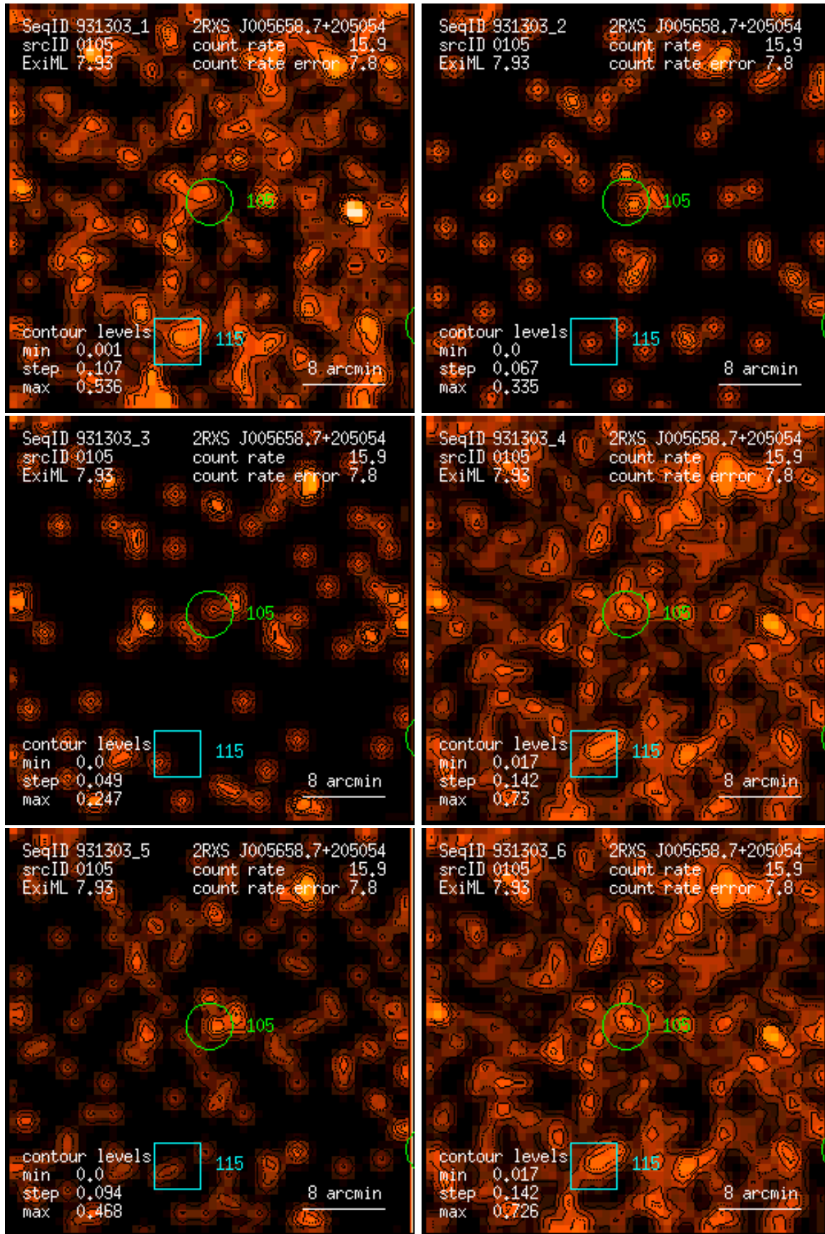
Figure 105: RASS 931303: detection 0105: band rate images, Gaussian filter: (1) PSPC channels 11 – 41, (2) 52 – 90, (3) 91 – 201, (4) 11 – 235, (5) 52 – 201, (6) 11 – 201. Broad band rates in counts/ks. Band rate contour levels in counts/ks/arcmin 2 .
