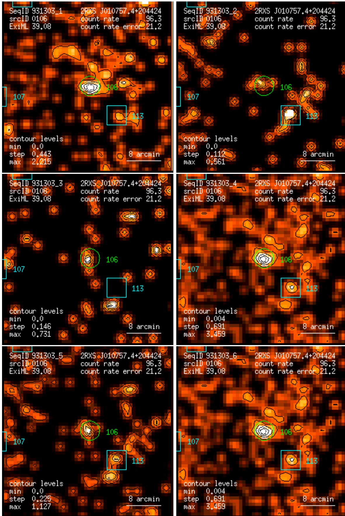
Figure 106: RASS 931303: detection 0106: band rate images, Gaussian filter: (1) PSPC channels 11 – 41, (2) 52 – 90, (3) 91 – 201, (4) 11 – 235, (5) 52 – 201, (6) 11 – 201. Broad band rates in counts/ks. Band rate contour levels in counts/ks/arcmin 2 .
