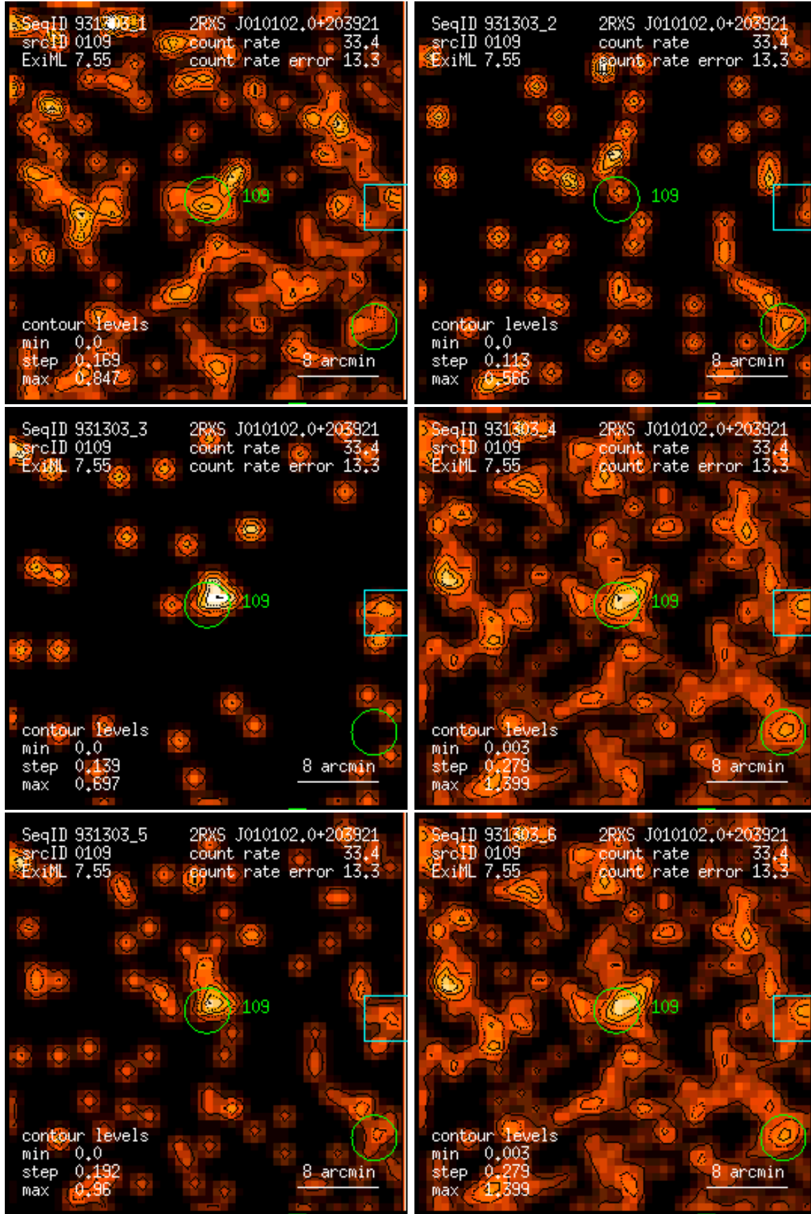
Figure 109: RASS 931303: detection 0109: band rate images, Gaussian filter: (1) PSPC channels 11 – 41, (2) 52 – 90, (3) 91 – 201, (4) 11 – 235, (5) 52 – 201, (6) 11 – 201. Broad band rates in counts/ks. Band rate contour levels in counts/ks/arcmin 2 .
