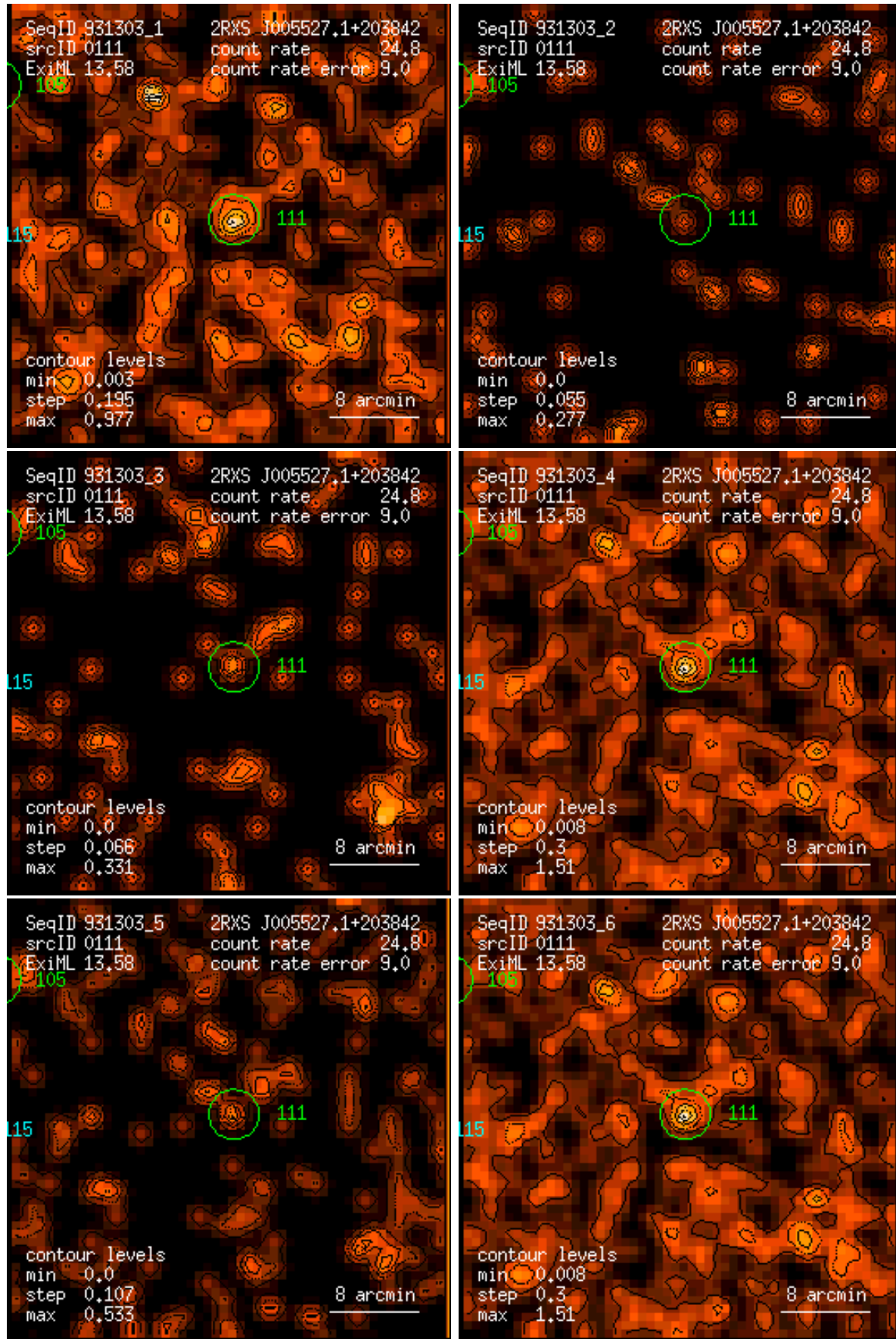
Figure 111: RASS 931303: detection 0111: band rate images, Gaussian filter: (1) PSPC channels 11 – 41, (2) 52 – 90, (3) 91 – 201, (4) 11 – 235, (5) 52 – 201, (6) 11 – 201. Broad band rates in counts/ks. Band rate contour levels in counts/ks/arcmin 2 .
