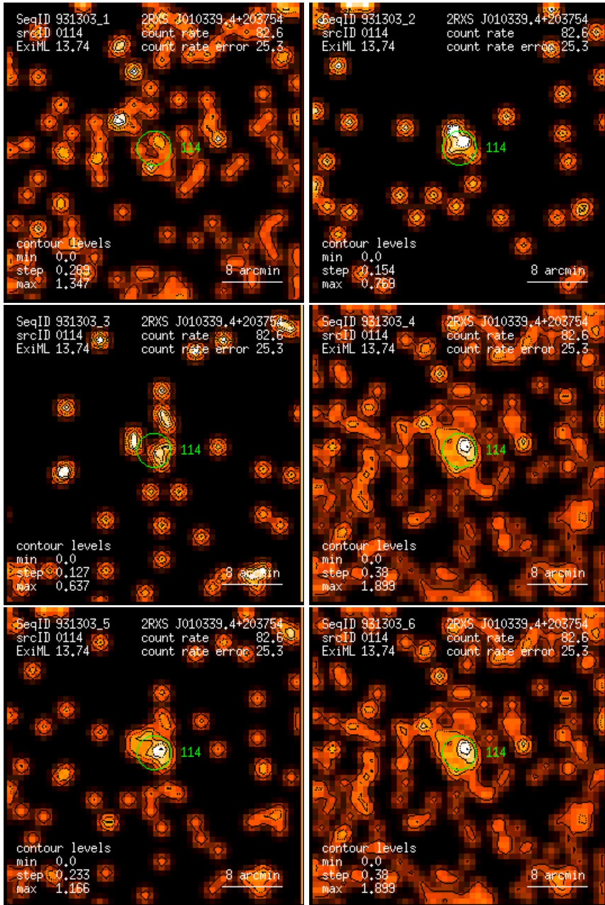
Figure 114: RASS 931303: detection 0114: band rate images, Gaussian filter: (1) PSPC channels 11 – 41, (2) 52 – 90, (3) 91 – 201, (4) 11 – 235, (5) 52 – 201, (6) 11 – 201. Broad band rates in counts/ks. Band rate contour levels in counts/ks/arcmin 2 .
