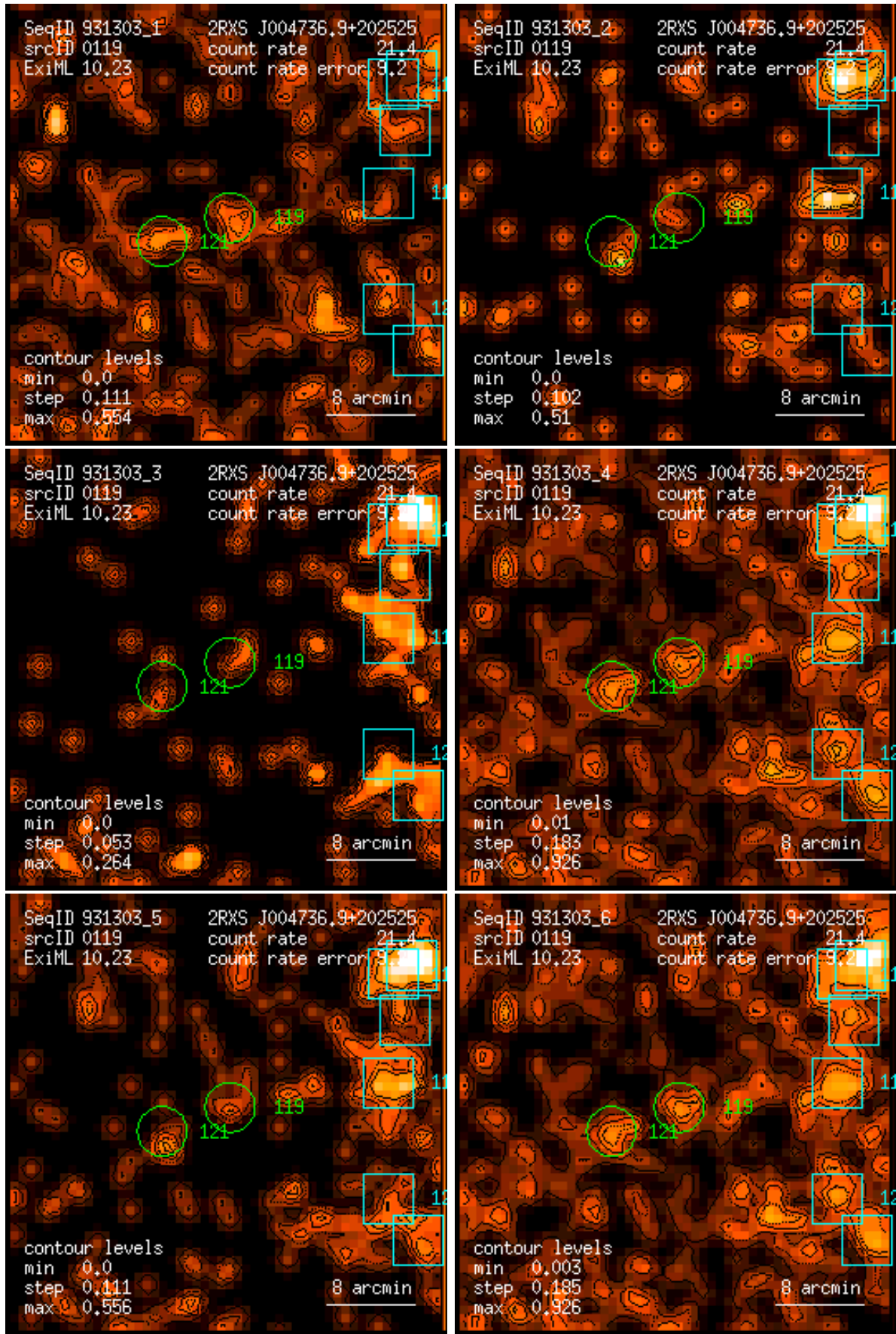
Figure 119: RASS 931303: detection 0119: band rate images, Gaussian filter: (1) PSPC channels 11 – 41, (2) 52 – 90, (3) 91 – 201, (4) 11 – 235, (5) 52 – 201, (6) 11 – 201. Broad band rates in counts/ks. Band rate contour levels in counts/ks/arcmin 2 .
