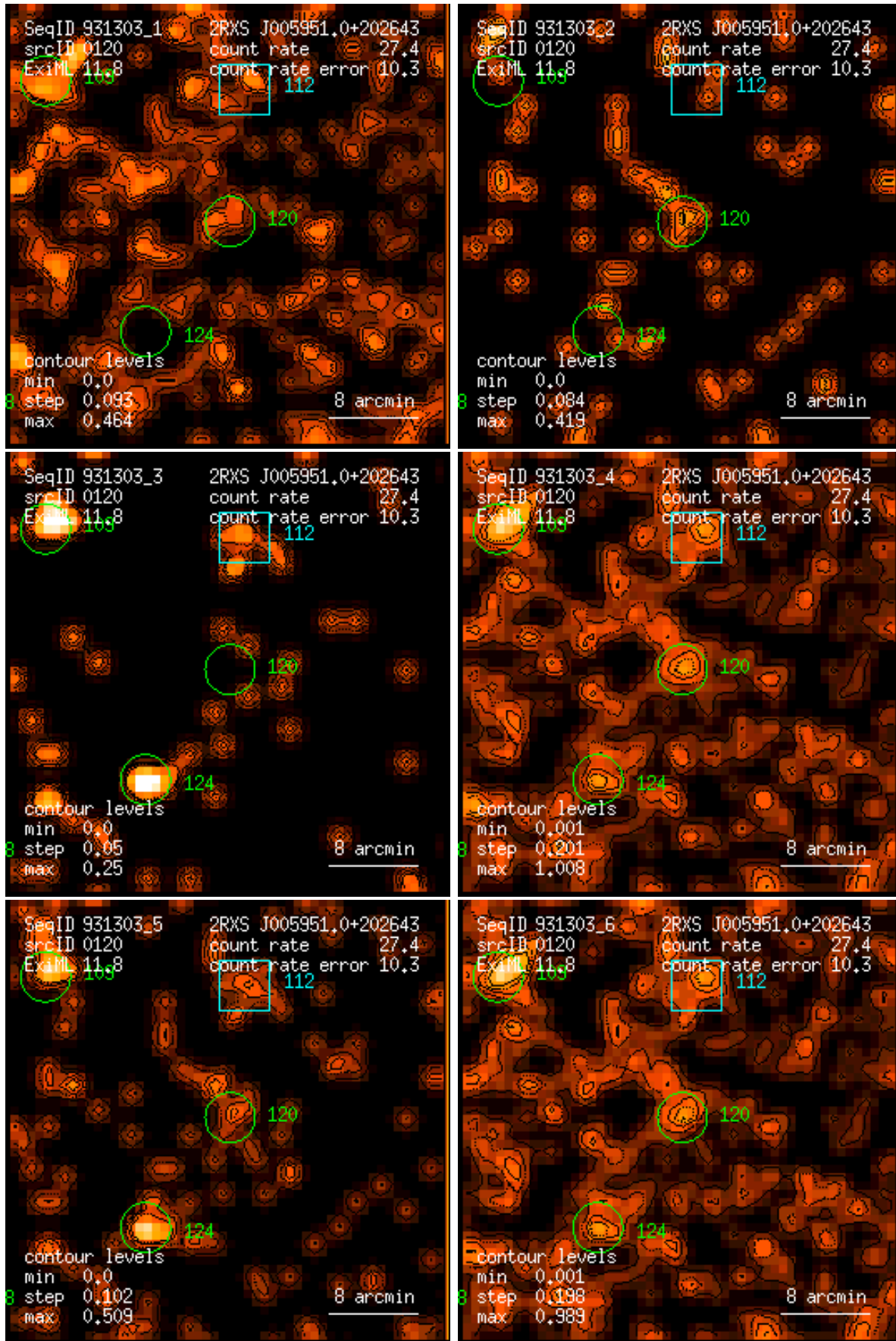
Figure 120: RASS 931303: detection 0120: band rate images, Gaussian filter: (1) PSPC channels 11 – 41, (2) 52 – 90, (3) 91 – 201, (4) 11 – 235, (5) 52 – 201, (6) 11 – 201. Broad band rates in counts/ks. Band rate contour levels in counts/ks/arcmin 2 .
