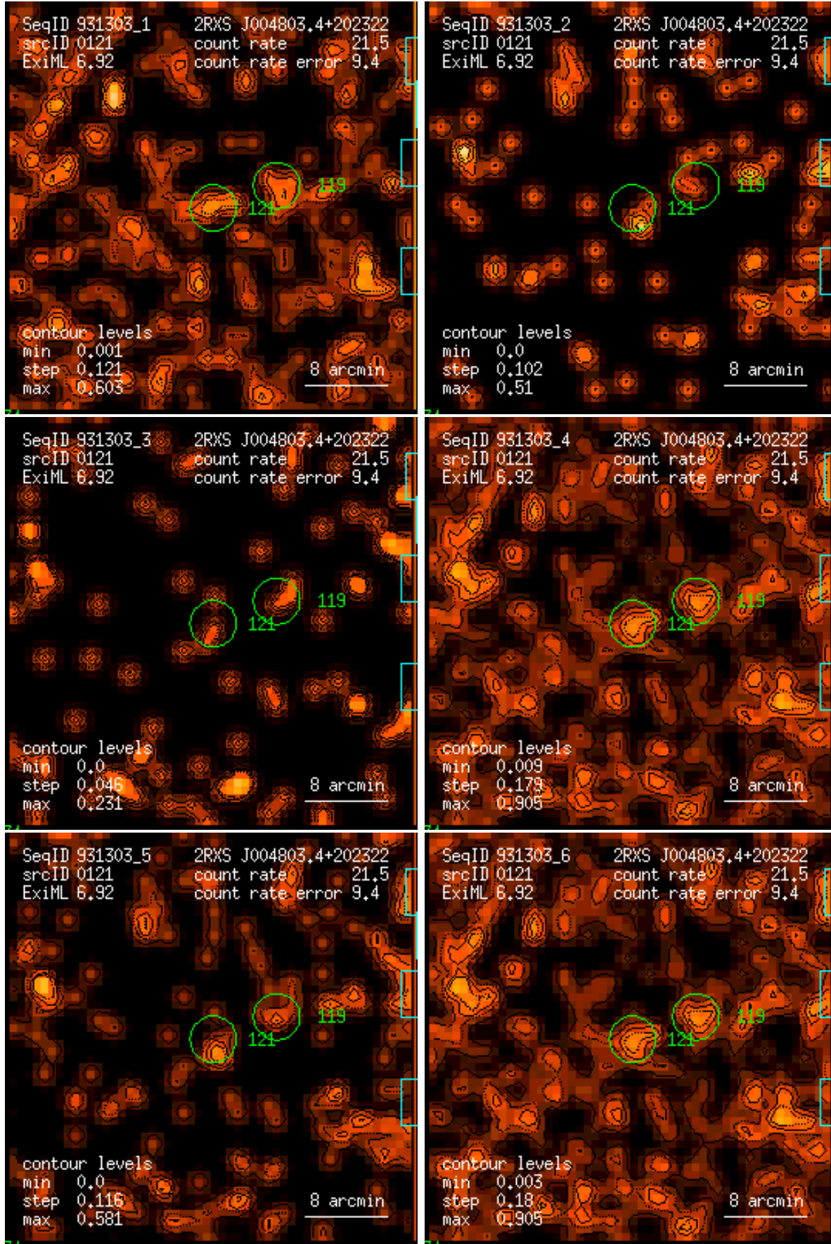
Figure 121: RASS 931303: detection 0121: band rate images, Gaussian filter: (1) PSPC channels 11 – 41, (2) 52 – 90, (3) 91 – 201, (4) 11 – 235, (5) 52 – 201, (6) 11 – 201. Broad band rates in counts/ks. Band rate contour levels in counts/ks/arcmin 2 .
