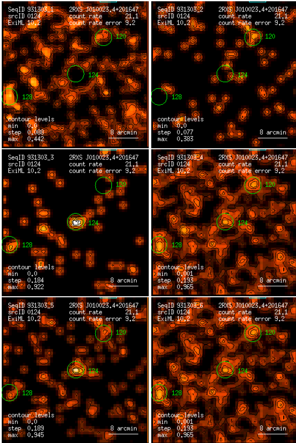
Figure 124: RASS 931303: detection 0124: band rate images, Gaussian filter: (1) PSPC channels 11 – 41, (2) 52 – 90, (3) 91 – 201, (4) 11 – 235, (5) 52 – 201, (6) 11 – 201. Broad band rates in counts/ks. Band rate contour levels in counts/ks/arcmin 2 .
