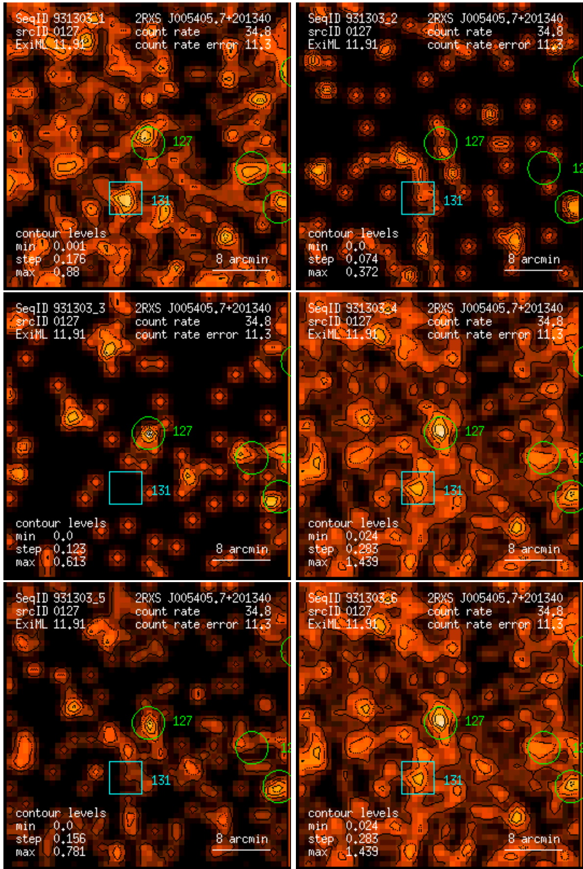
Figure 127: RASS 931303: detection 0127: band rate images, Gaussian filter: (1) PSPC channels 11 – 41, (2) 52 – 90, (3) 91 – 201, (4) 11 – 235, (5) 52 – 201, (6) 11 – 201. Broad band rates in counts/ks. Band rate contour levels in counts/ks/arcmin 2 .
