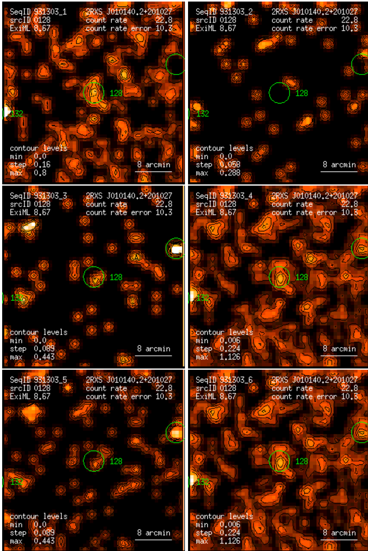
Figure 128: RASS 931303: detection 0128: band rate images, Gaussian filter: (1) PSPC channels 11 – 41, (2) 52 – 90, (3) 91 – 201, (4) 11 – 235, (5) 52 – 201, (6) 11 – 201. Broad band rates in counts/ks. Band rate contour levels in counts/ks/arcmin 2 .
