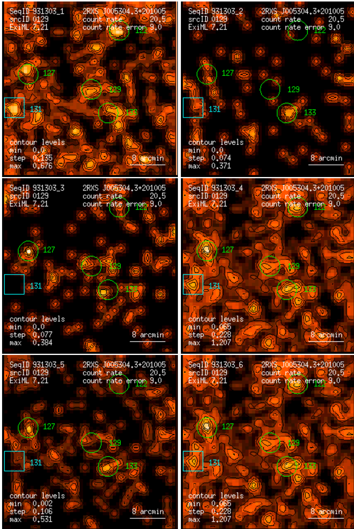
Figure 129: RASS 931303: detection 0129: band rate images, Gaussian filter: (1) PSPC channels 11 – 41, (2) 52 – 90, (3) 91 – 201, (4) 11 – 235, (5) 52 – 201, (6) 11 – 201. Broad band rates in counts/ks. Band rate contour levels in counts/ks/arcmin 2 .
