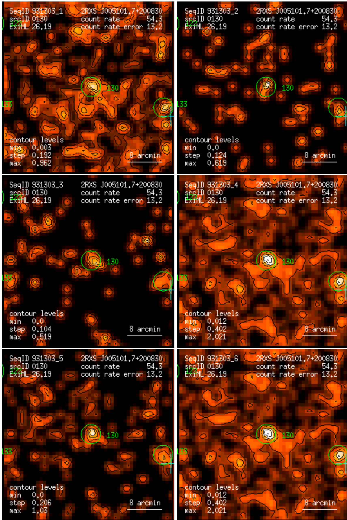
Figure 130: RASS 931303: detection 0130: band rate images, Gaussian filter: (1) PSPC channels 11 – 41, (2) 52 – 90, (3) 91 – 201, (4) 11 – 235, (5) 52 – 201, (6) 11 – 201. Broad band rates in counts/ks. Band rate contour levels in counts/ks/arcmin 2 .
