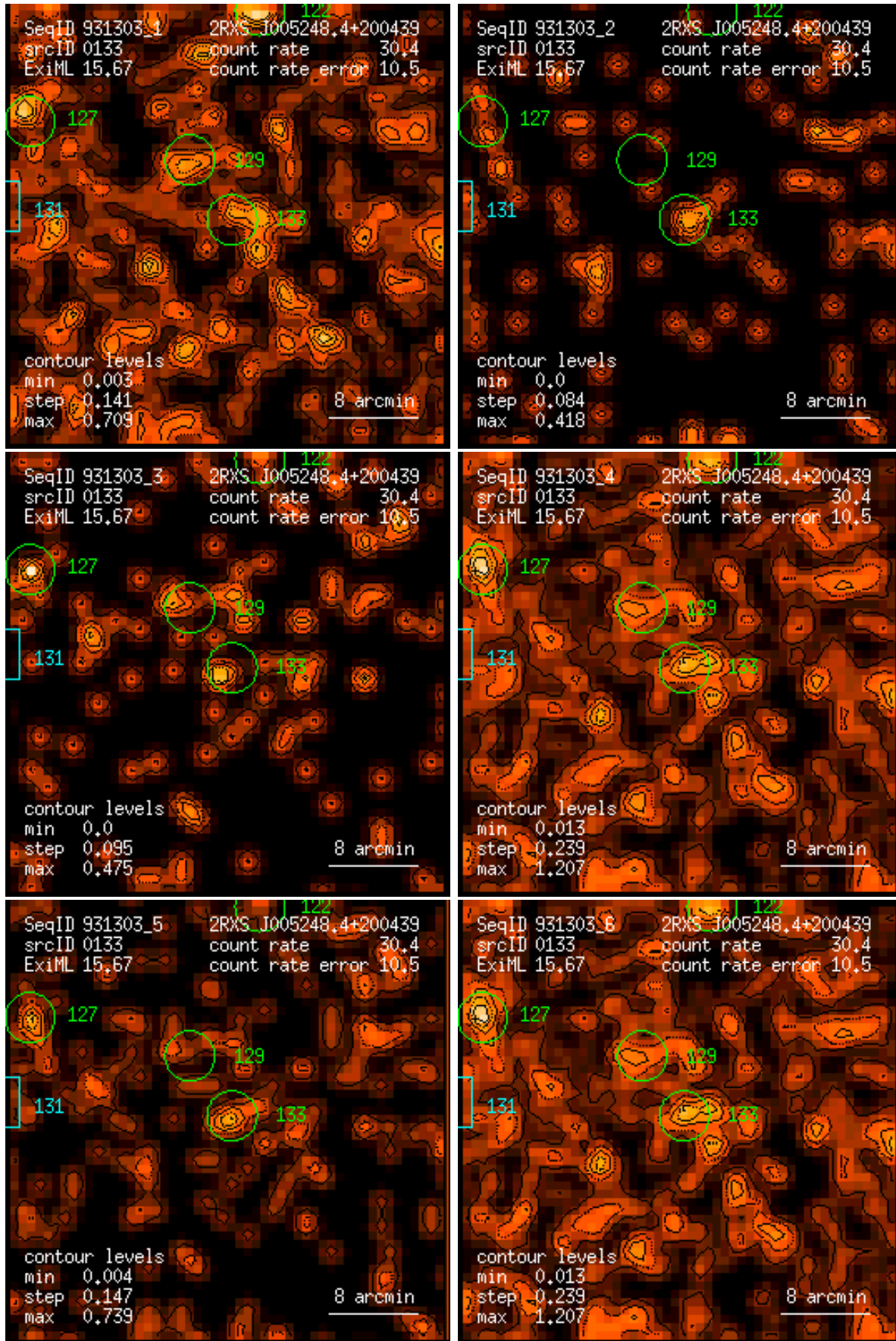
Figure 133: RASS 931303: detection 0133: band rate images, Gaussian filter: (1) PSPC channels 11 – 41, (2) 52 – 90, (3) 91 – 201, (4) 11 – 235, (5) 52 – 201, (6) 11 – 201. Broad band rates in counts/ks. Band rate contour levels in counts/ks/arcmin 2 .
