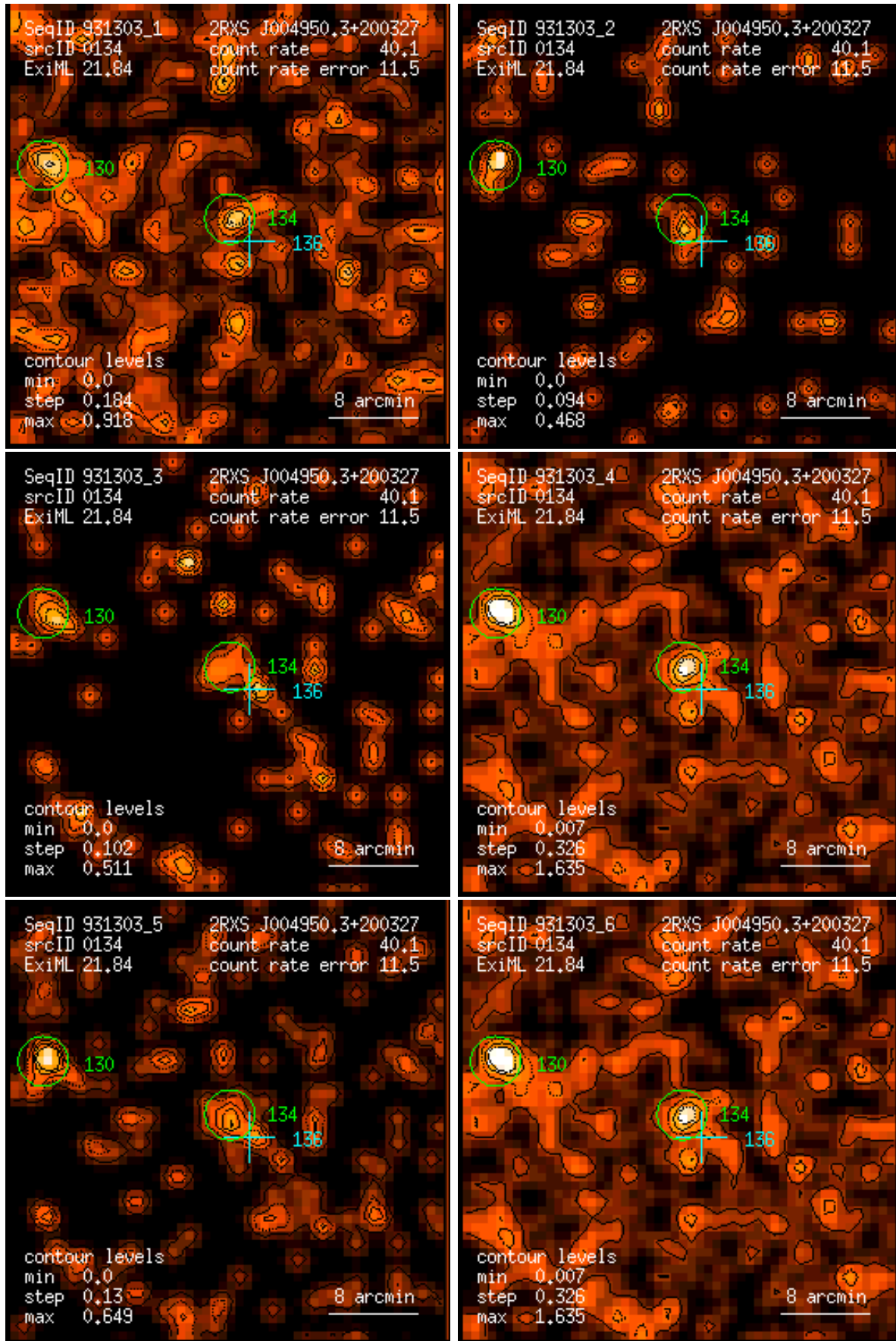
Figure 134: RASS 931303: detection 0134: band rate images, Gaussian filter: (1) PSPC channels 11 – 41, (2) 52 – 90, (3) 91 – 201, (4) 11 – 235, (5) 52 – 201, (6) 11 – 201. Broad band rates in counts/ks. Band rate contour levels in counts/ks/arcmin 2 .
