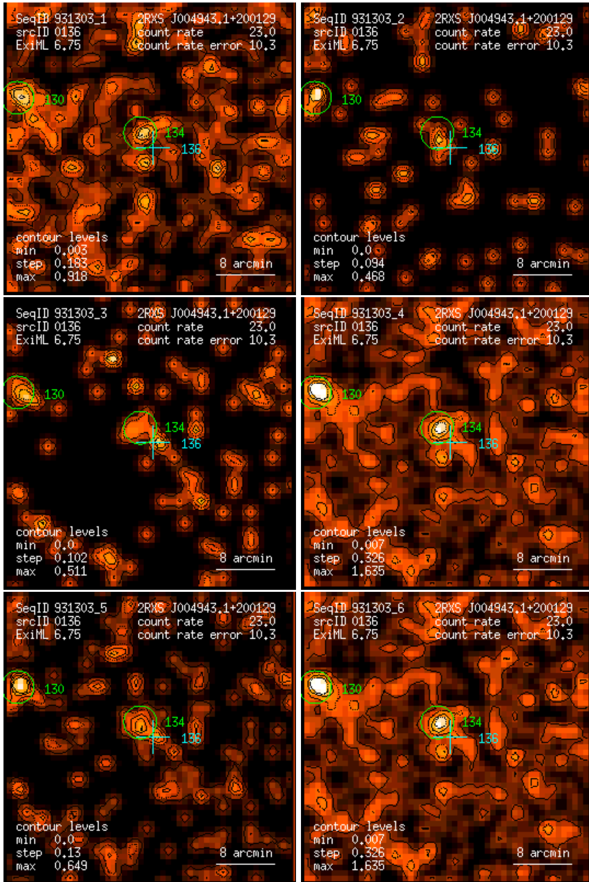
Figure 136: RASS 931303: detection 0136: band rate images, Gaussian filter: (1) PSPC channels 11 – 41, (2) 52 – 90, (3) 91 – 201, (4) 11 – 235, (5) 52 – 201, (6) 11 – 201. Broad band rates in counts/ks. Band rate contour levels in counts/ks/arcmin 2 .
