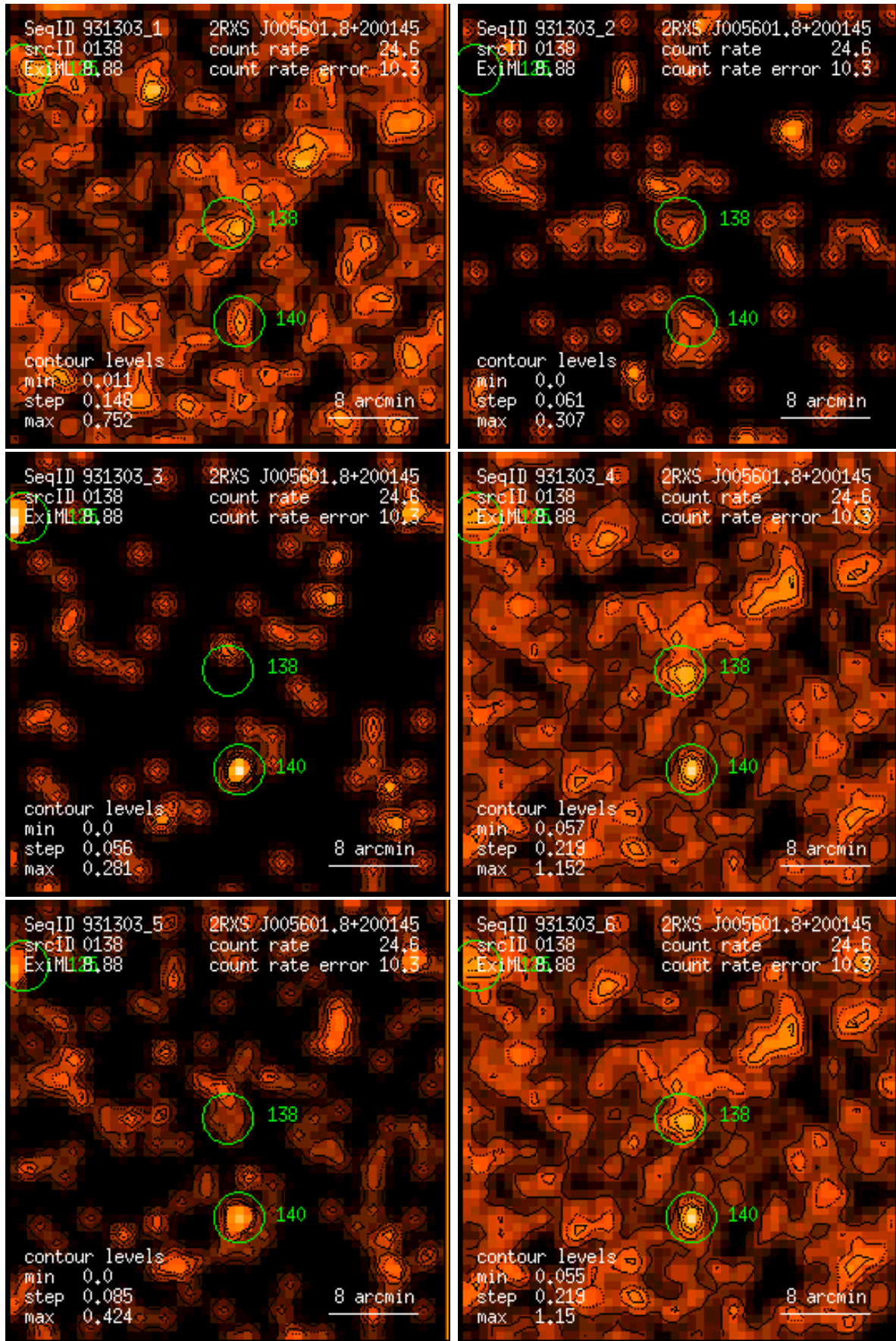
Figure 138: RASS 931303: detection 0138: band rate images, Gaussian filter: (1) PSPC channels 11 – 41, (2) 52 – 90, (3) 91 – 201, (4) 11 – 235, (5) 52 – 201, (6) 11 – 201. Broad band rates in counts/ks. Band rate contour levels in counts/ks/arcmin 2 .
