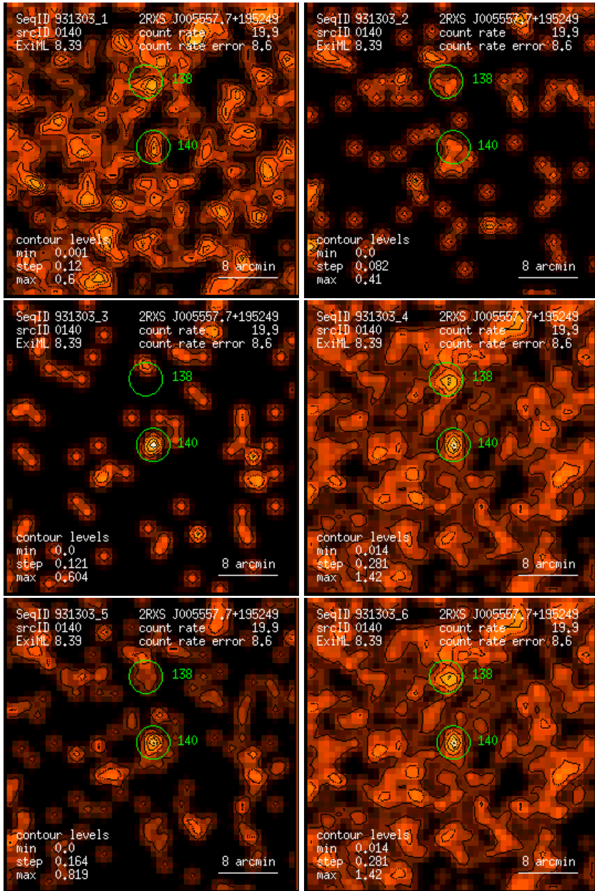
Figure 140: RASS 931303: detection 0140: band rate images, Gaussian filter: (1) PSPC channels 11 – 41, (2) 52 – 90, (3) 91 – 201, (4) 11 – 235, (5) 52 – 201, (6) 11 – 201. Broad band rates in counts/ks. Band rate contour levels in counts/ks/arcmin 2 .
