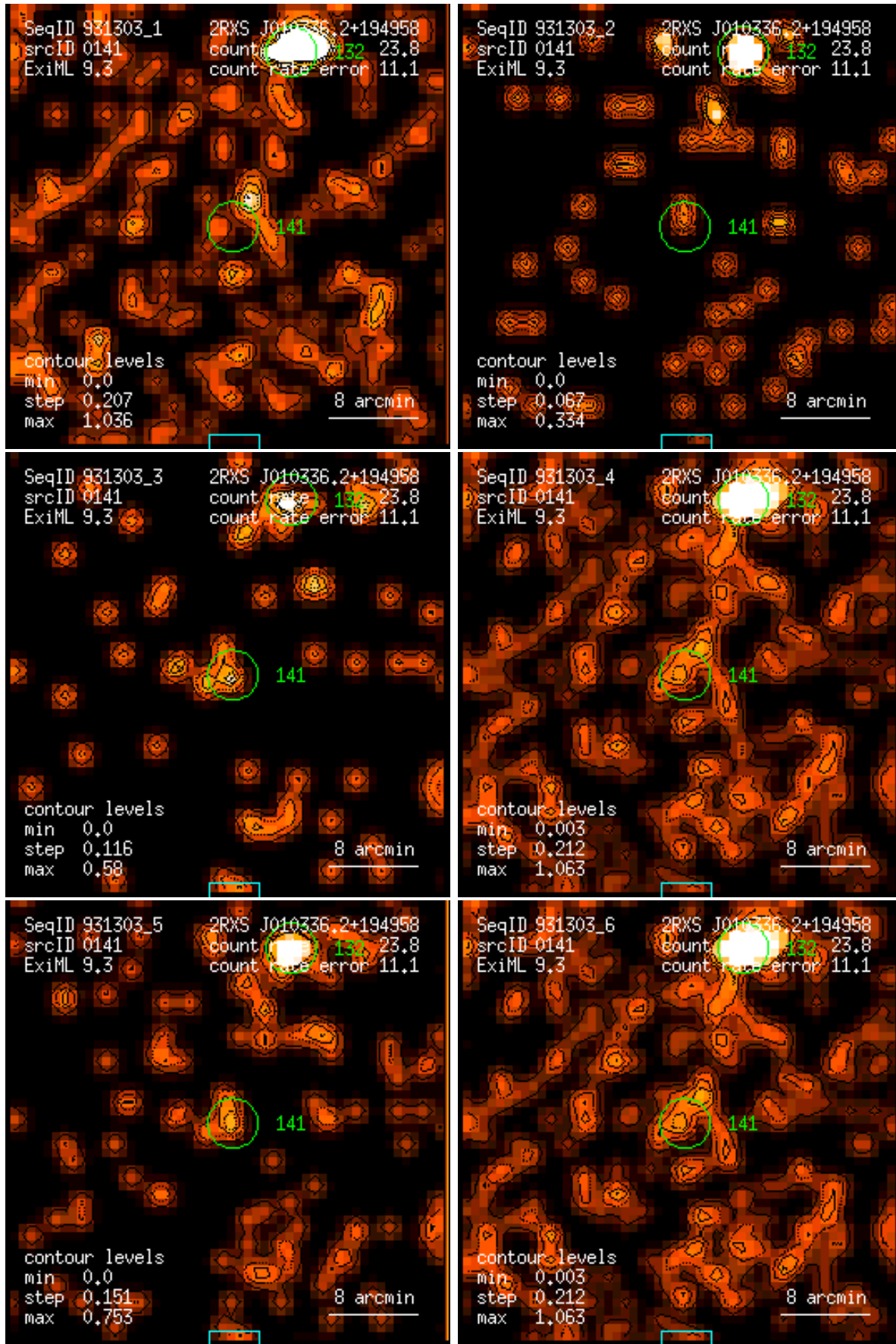
Figure 141: RASS 931303: detection 0141: band rate images, Gaussian filter: (1) PSPC channels 11 – 41, (2) 52 – 90, (3) 91 – 201, (4) 11 – 235, (5) 52 – 201, (6) 11 – 201. Broad band rates in counts/ks. Band rate contour levels in counts/ks/arcmin 2 .
