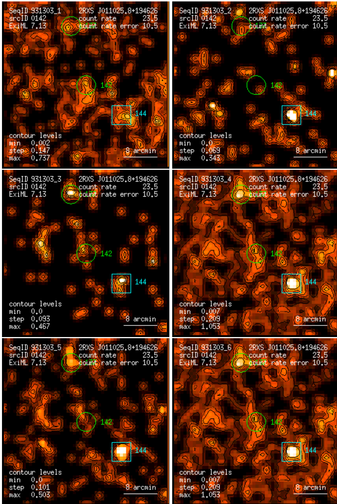
Figure 142: RASS 931303: detection 0142: band rate images, Gaussian filter: (1) PSPC channels 11 – 41, (2) 52 – 90, (3) 91 – 201, (4) 11 – 235, (5) 52 – 201, (6) 11 – 201. Broad band rates in counts/ks. Band rate contour levels in counts/ks/arcmin 2 .
