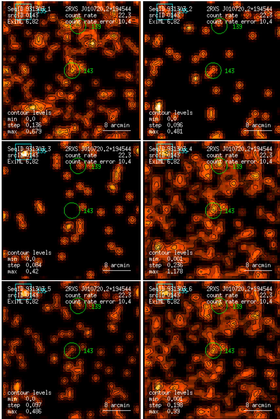
Figure 143: RASS 931303: detection 0143: band rate images, Gaussian filter: (1) PSPC channels 11 – 41, (2) 52 – 90, (3) 91 – 201, (4) 11 – 235, (5) 52 – 201, (6) 11 – 201. Broad band rates in counts/ks. Band rate contour levels in counts/ks/arcmin 2 .
