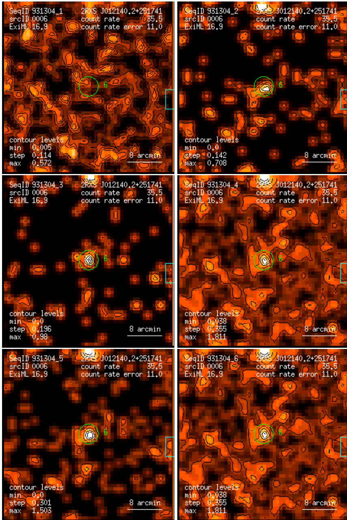
Figure 6: RASS 931304: detection 0006: band rate images, Gaussian filter: (1) PSPC channels 11 – 41, (2) 52 – 90, (3) 91 – 201, (4) 11 – 235, (5) 52 – 201, (6) 11 – 201. Broad band rates in counts/ks. Band rate contour levels in counts/ks/arcmin 2 .
