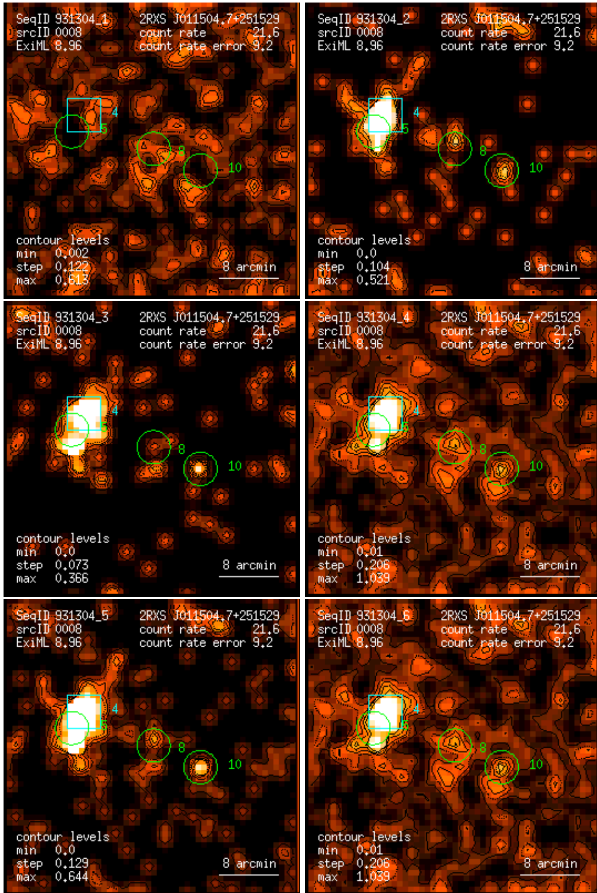
Figure 8: RASS 931304: detection 0008: band rate images, Gaussian filter: (1) PSPC channels 11 – 41, (2) 52 – 90, (3) 91 – 201, (4) 11 – 235, (5) 52 – 201, (6) 11 – 201. Broad band rates in counts/ks. Band rate contour levels in counts/ks/arcmin 2 .
