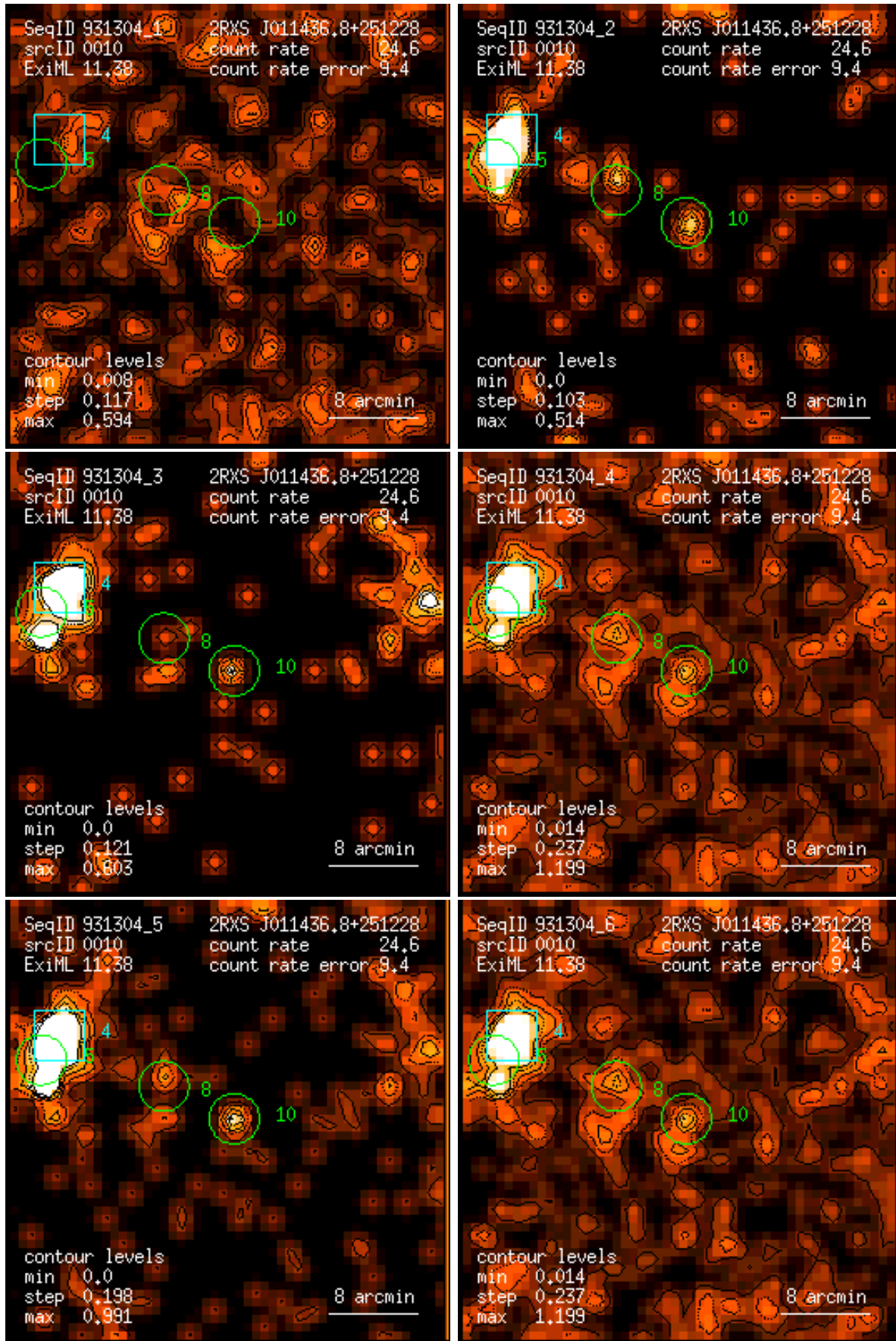
Figure 10: RASS 931304: detection 0010: band rate images, Gaussian filter: (1) PSPC channels 11 – 41, (2) 52 – 90, (3) 91 – 201, (4) 11 – 235, (5) 52 – 201, (6) 11 – 201. Broad band rates in counts/ks. Band rate contour levels in counts/ks/arcmin 2 .
