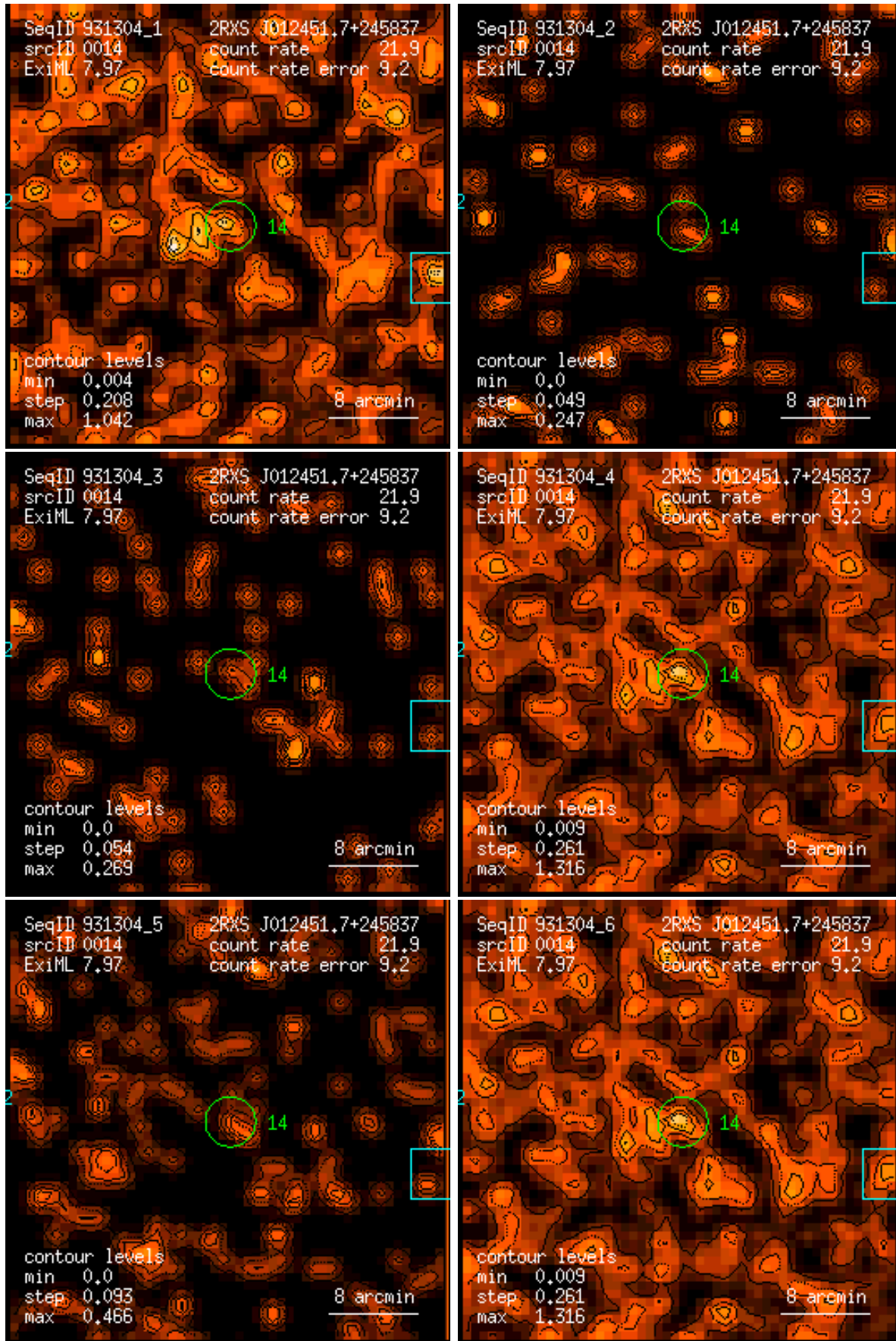
Figure 14: RASS 931304: detection 0014: band rate images, Gaussian filter: (1) PSPC channels 11 – 41, (2) 52 – 90, (3) 91 – 201, (4) 11 – 235, (5) 52 – 201, (6) 11 – 201. Broad band rates in counts/ks. Band rate contour levels in counts/ks/arcmin 2 .
