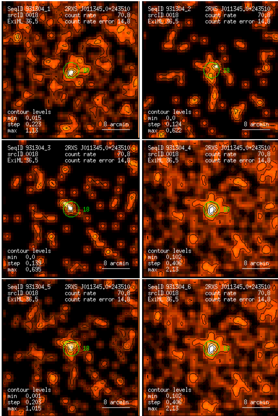
Figure 18: RASS 931304: detection 0018: band rate images, Gaussian filter: (1) PSPC channels 11 – 41, (2) 52 – 90, (3) 91 – 201, (4) 11 – 235, (5) 52 – 201, (6) 11 – 201. Broad band rates in counts/ks. Band rate contour levels in counts/ks/arcmin 2 .
