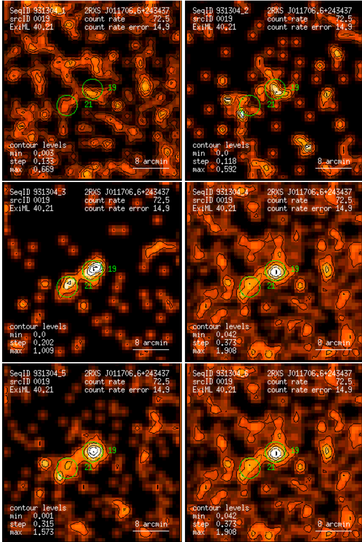
Figure 19: RASS 931304: detection 0019: band rate images, Gaussian filter: (1) PSPC channels 11 – 41, (2) 52 – 90, (3) 91 – 201, (4) 11 – 235, (5) 52 – 201, (6) 11 – 201. Broad band rates in counts/ks. Band rate contour levels in counts/ks/arcmin 2 .
