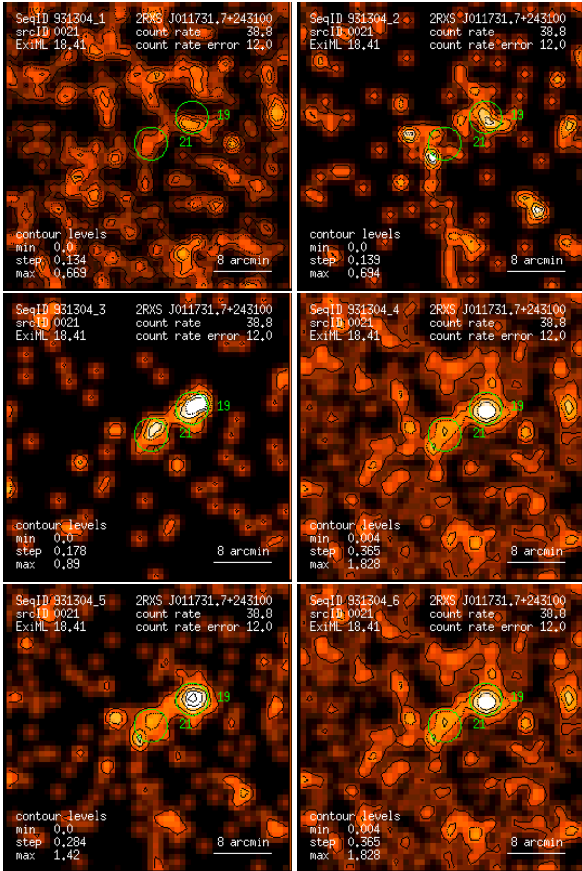
Figure 21: RASS 931304: detection 0021: band rate images, Gaussian filter: (1) PSPC channels 11 – 41, (2) 52 – 90, (3) 91 – 201, (4) 11 – 235, (5) 52 – 201, (6) 11 – 201. Broad band rates in counts/ks. Band rate contour levels in counts/ks/arcmin 2 .
