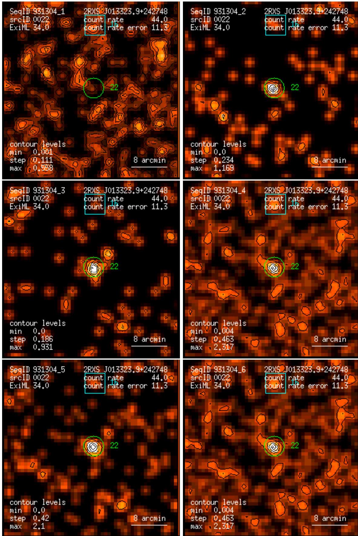
Figure 22: RASS 931304: detection 0022: band rate images, Gaussian filter: (1) PSPC channels 11 – 41, (2) 52 – 90, (3) 91 – 201, (4) 11 – 235, (5) 52 – 201, (6) 11 – 201. Broad band rates in counts/ks. Band rate contour levels in counts/ks/arcmin 2 .
