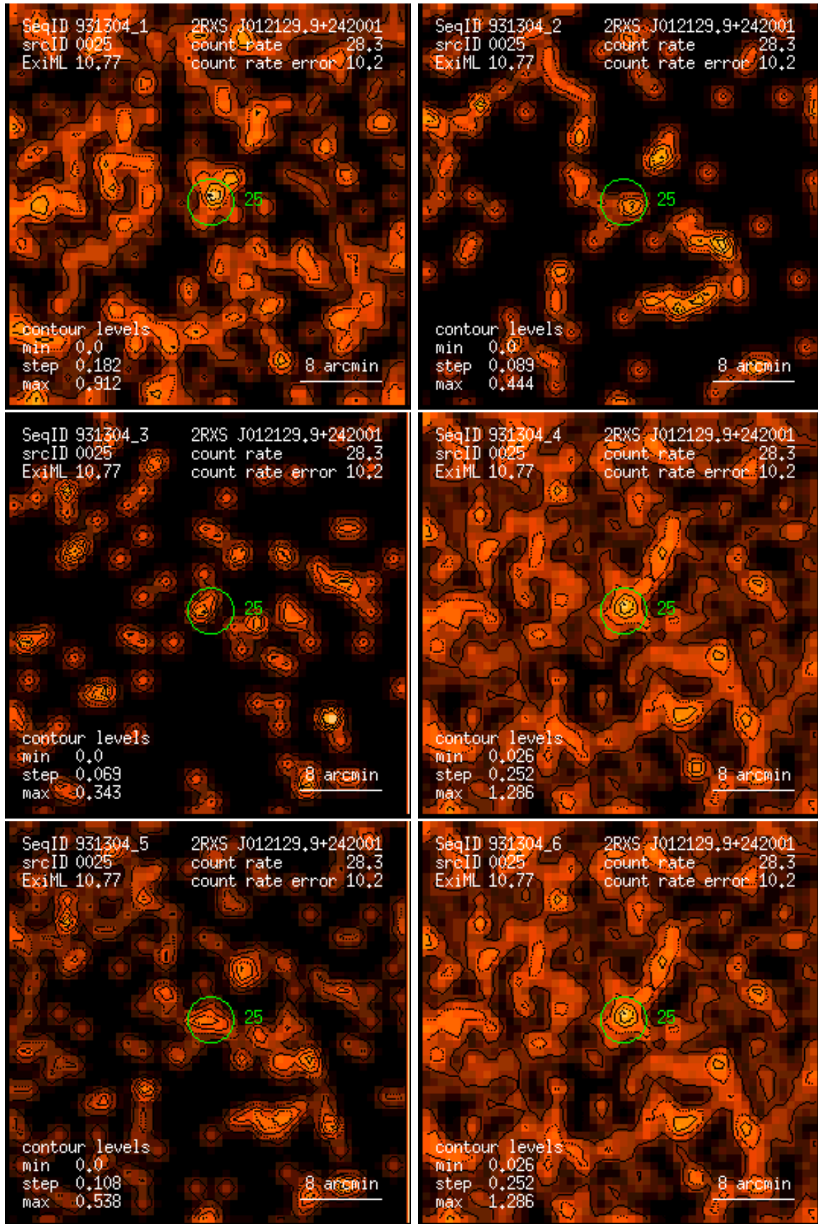
Figure 25: RASS 931304: detection 0025: band rate images, Gaussian filter: (1) PSPC channels 11 – 41, (2) 52 – 90, (3) 91 – 201, (4) 11 – 235, (5) 52 – 201, (6) 11 – 201. Broad band rates in counts/ks. Band rate contour levels in counts/ks/arcmin 2 .
