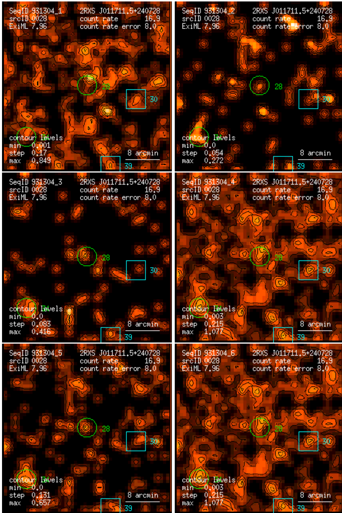
Figure 28: RASS 931304: detection 0028: band rate images, Gaussian filter: (1) PSPC channels 11 – 41, (2) 52 – 90, (3) 91 – 201, (4) 11 – 235, (5) 52 – 201, (6) 11 – 201. Broad band rates in counts/ks. Band rate contour levels in counts/ks/arcmin 2 .
