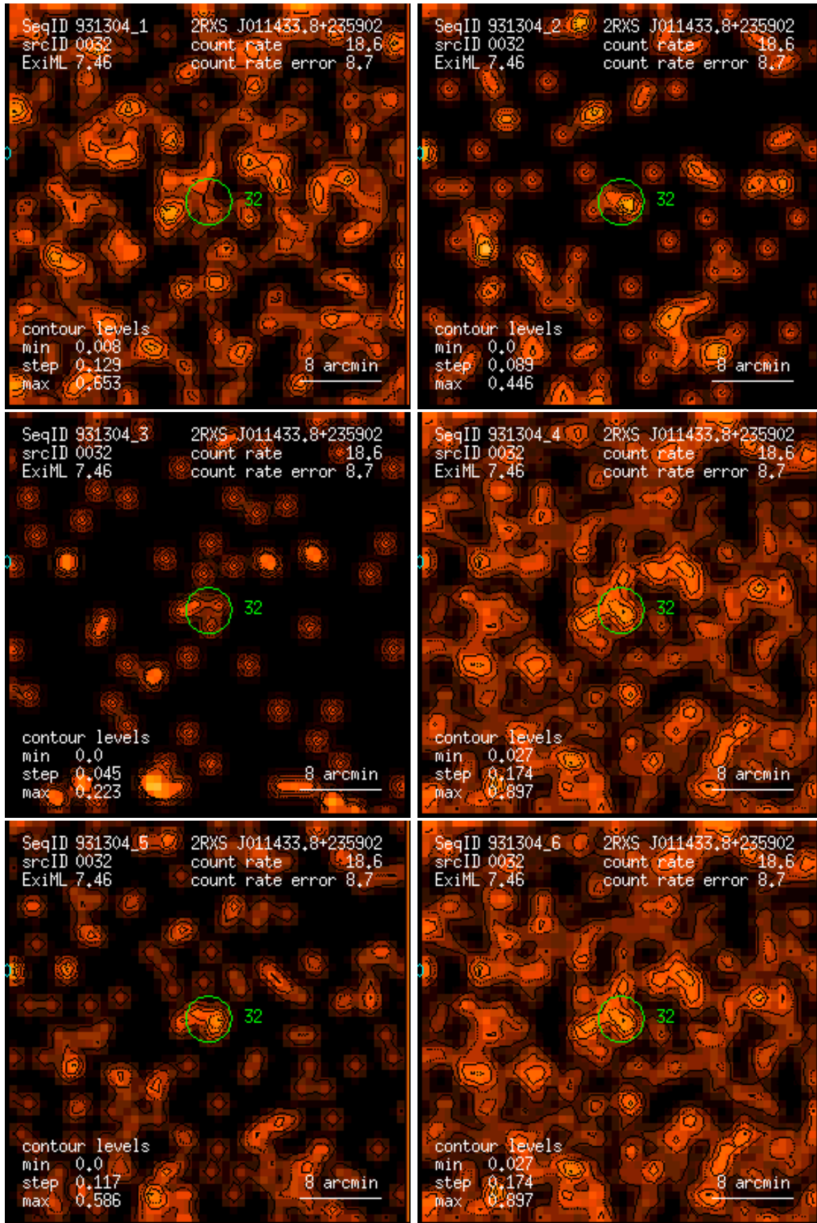
Figure 32: RASS 931304: detection 0032: band rate images, Gaussian filter: (1) PSPC channels 11 – 41, (2) 52 – 90, (3) 91 – 201, (4) 11 – 235, (5) 52 – 201, (6) 11 – 201. Broad band rates in counts/ks. Band rate contour levels in counts/ks/arcmin 2 .
