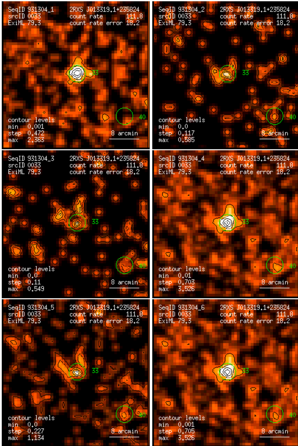
Figure 33: RASS 931304: detection 0033: band rate images, Gaussian filter: (1) PSPC channels 11 – 41, (2) 52 – 90, (3) 91 – 201, (4) 11 – 235, (5) 52 – 201, (6) 11 – 201. Broad band rates in counts/ks. Band rate contour levels in counts/ks/arcmin 2 .
